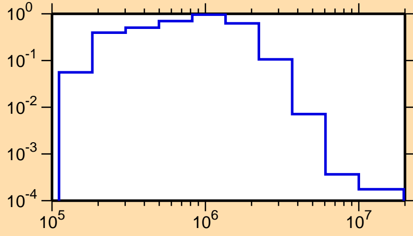
\sigma vs. E for ^{141}\text{Pr}(n,n_1)
