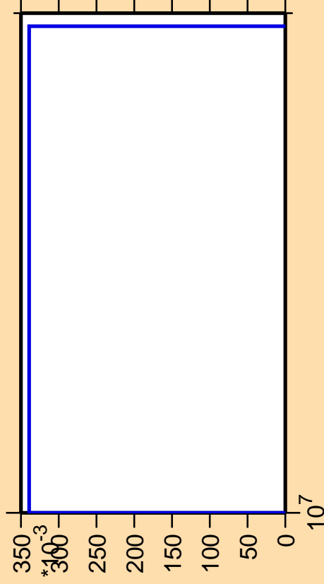
\Delta\sigma/\sigma vs. E for ^{141}\text{Pr}(\text{mt117})
