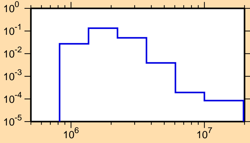
\sigma vs. E for ^{141}\text{Pr}(n,n_3)
