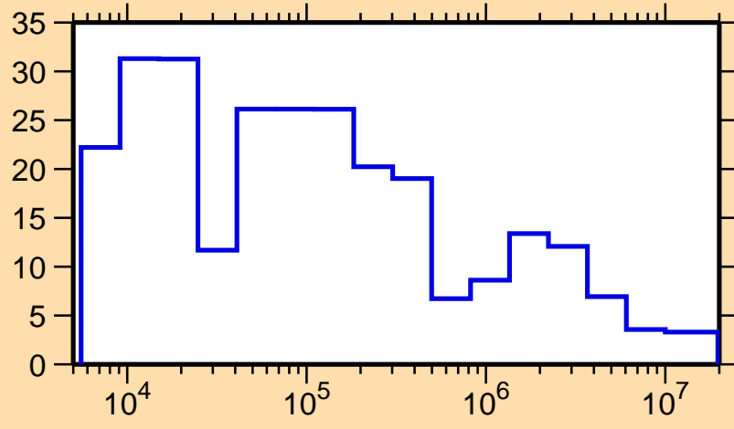
\Delta\sigma/\sigma vs. E for ^{141}\text{Pr}(n,\text{tot.})
