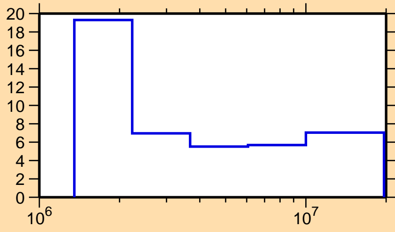
\Delta\sigma/\sigma vs. E for ^{141}\text{Pr}(n,\text{nonel.})
