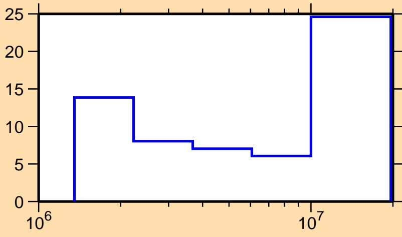
\Delta\sigma/\sigma vs. E for ^{141}\text{Pr}(n,n\text{cont.})
