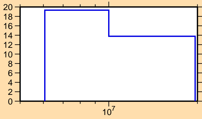
\Delta\sigma/\sigma vs. E for ^{141}\text{Pr}(n,2n)
