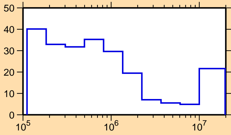
\Delta\sigma/\sigma vs. E for ^{141}\text{Pr}(n,\text{inel.})
