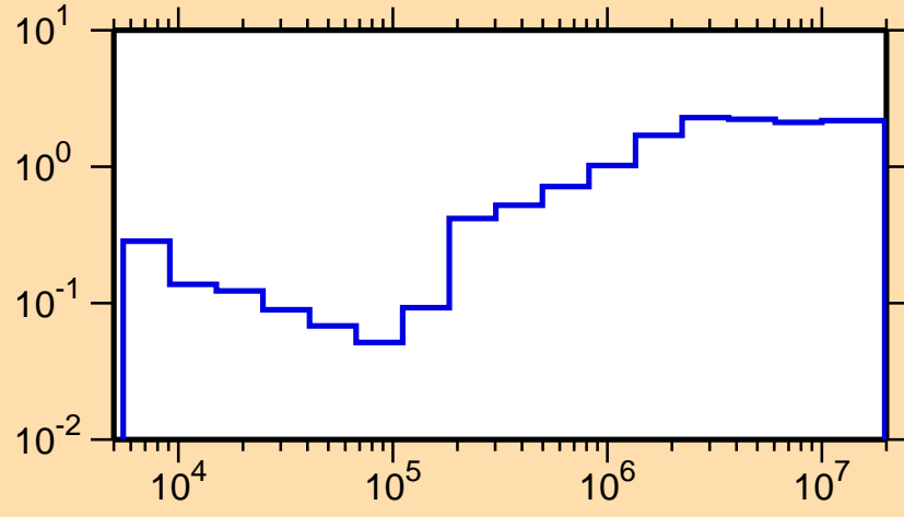
\sigma vs. E for ^{141}\text{Pr}(n,\text{nonel.})
