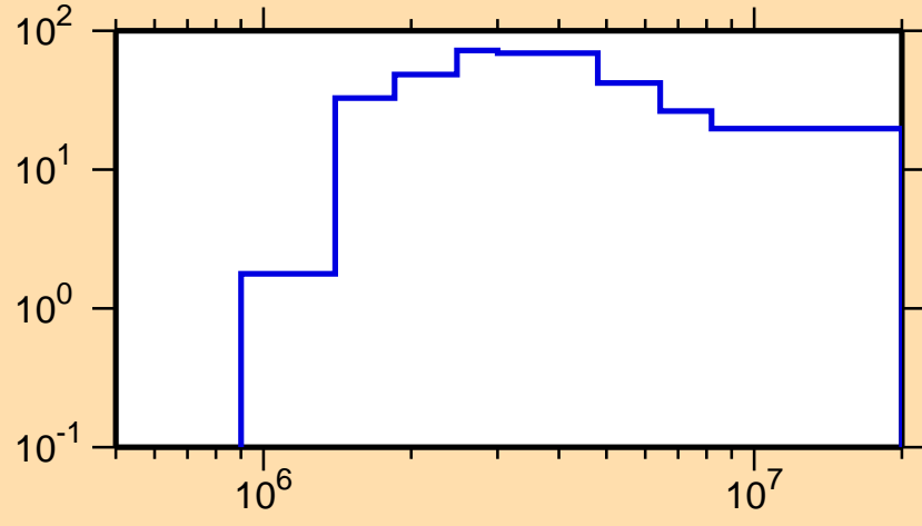
\Delta\sigma/\sigma vs. E for ^{141}\text{Pr}(n,p)
