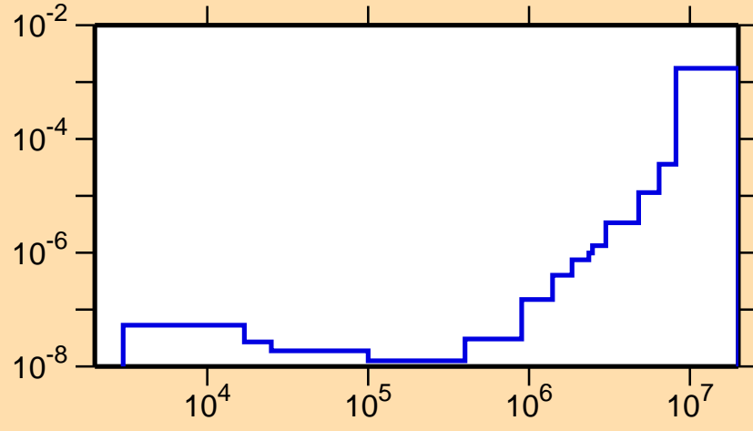
\sigma vs. E for ^{141}\text{Pr}(n,\alpha)
