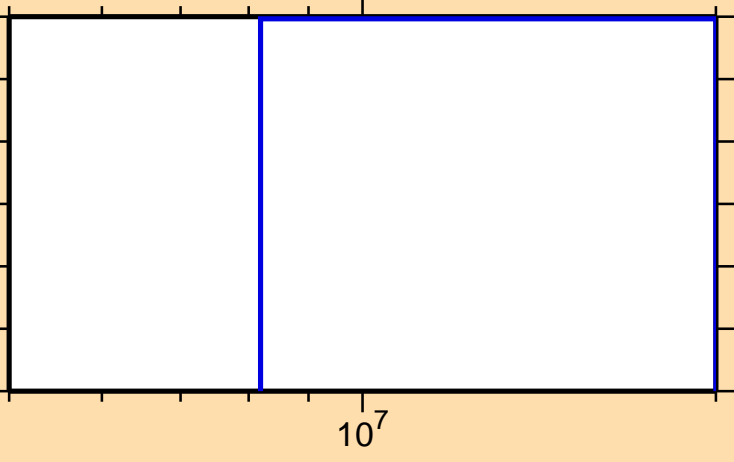
\sigma vs. E for ^{141}\text{Pr}(n,\text{He3})
