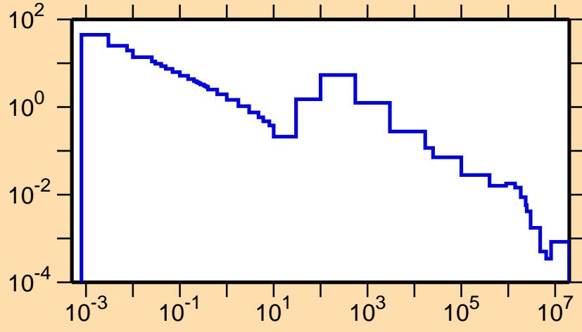
\sigma vs. E for ^{141}\text{Pr}(n,\gamma)
