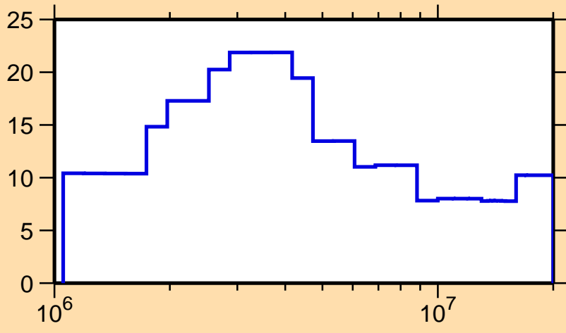
\Delta\sigma/\sigma vs. E for ^{142}\text{Pr}(n, el.)
