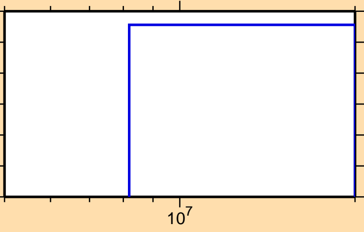
\sigma vs. E for ^{142}\text{Pr}(n,\text{He3})
