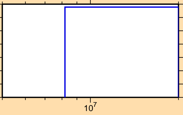
\sigma vs. E for ^{142}\text{Pr}(n,\text{nd})
