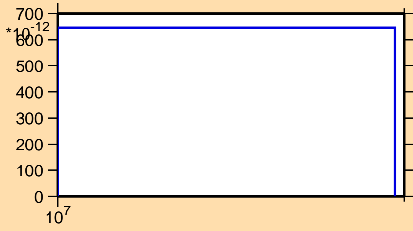
\sigma vs. E for ^{142}\text{Pr}(n,\text{He3})
