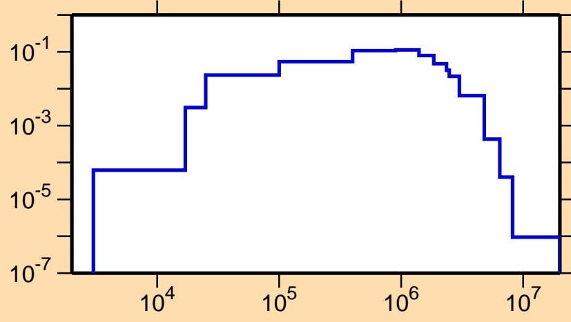
\sigma vs. E for ^{142}\text{Pr}(n,n_2)
