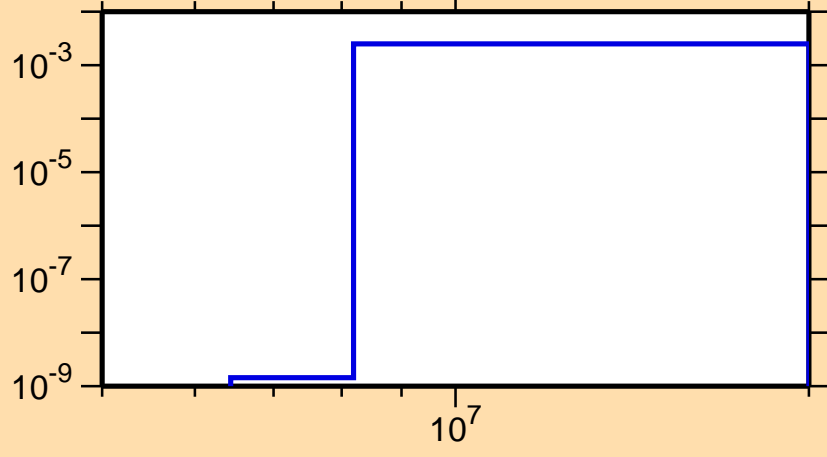
\sigma vs. E for ^{142}\text{Pr}(n,np)
