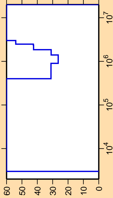
\Delta\sigma/\sigma vs. E for ^{142}\text{Pr}(n,n_2)
