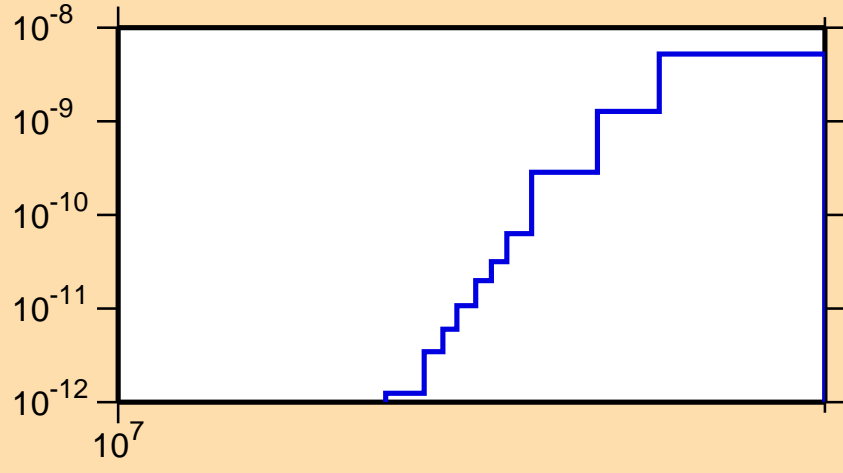
\sigma vs. E for ^{143}\text{Pr}(\text{mt117})
