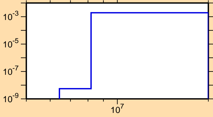
\sigma vs. E for ^{143}\text{Pr}(n,d)
