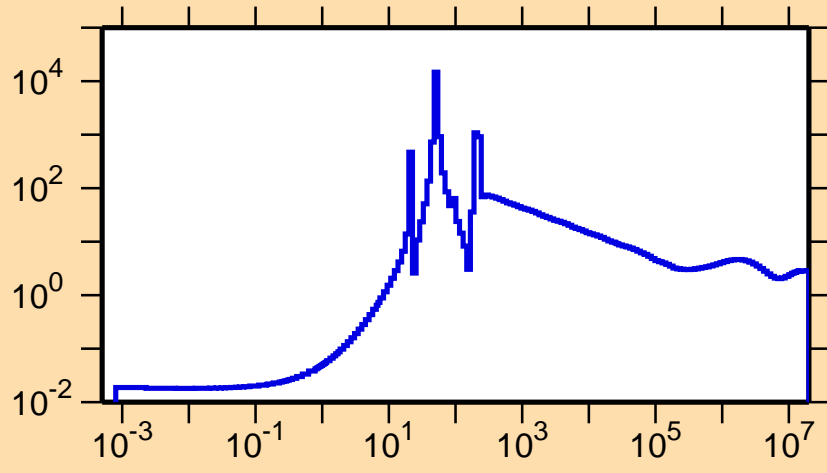
\sigma vs. E for ^{144}\text{Pr}(n,\text{el.})
