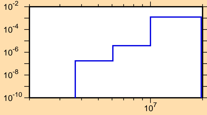
\sigma vs. E for ^{144}\text{Pr}(n,n\alpha)
