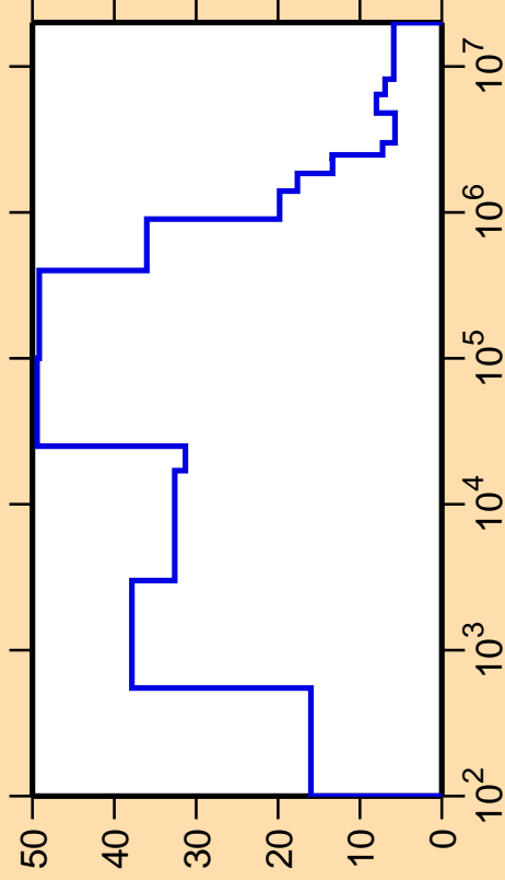
\Delta\sigma/\sigma vs. E for ^{144}\text{Pr}(n,\text{nonel.})
