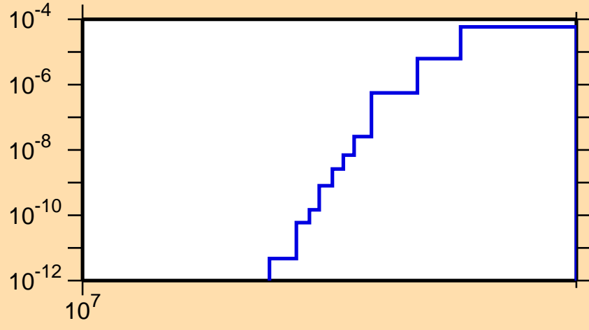
\sigma vs. E for ^{144}\text{Pr}(n,nt)
