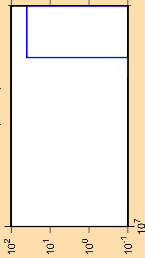
\Delta\sigma/\sigma vs. E for ^{144}\text{Pr}(n,3n\alpha)
