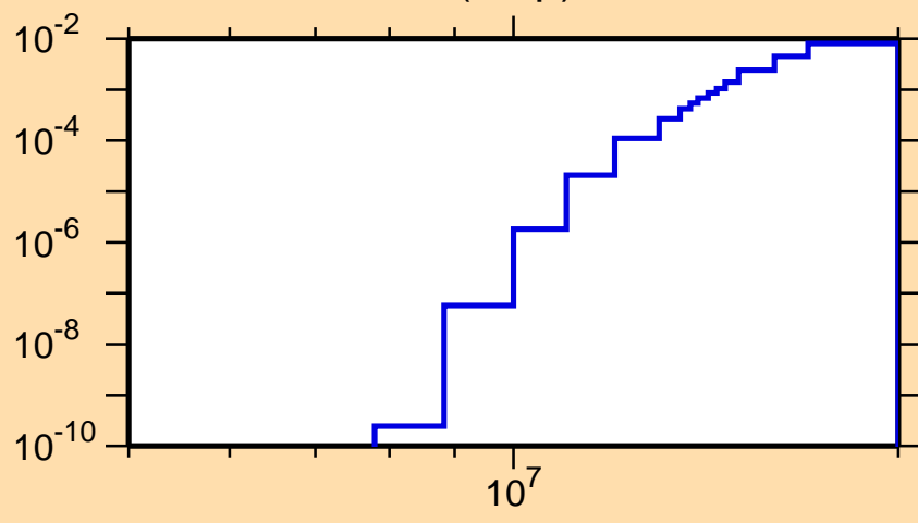
\sigma vs. E for ^{144}\text{Pr}(n,np)
