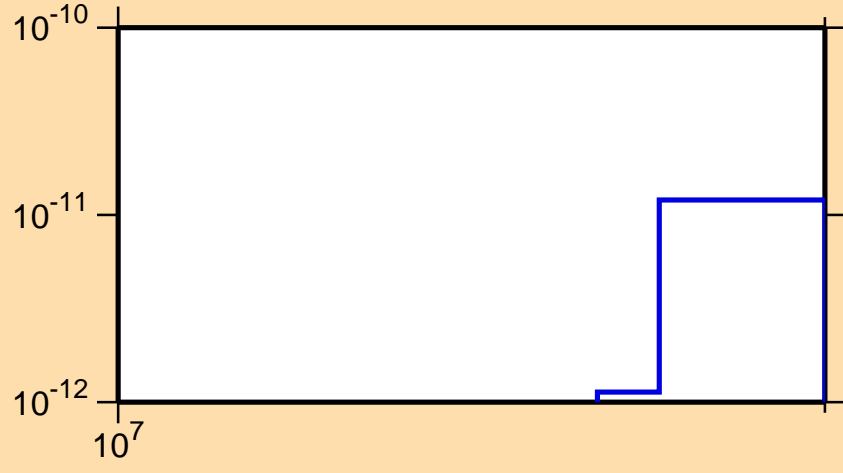
\sigma vs. E for ^{144}\text{Pr}(\text{mt } 45)
