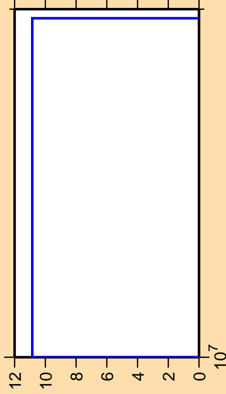
\Delta\sigma/\sigma vs. E for ^{144}\text{Pr}(\text{mt117})
