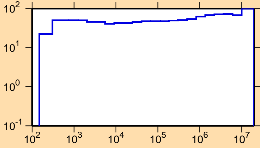
\Delta\sigma/\sigma vs. E for ^{144}\text{Pr}(n,\gamma)
