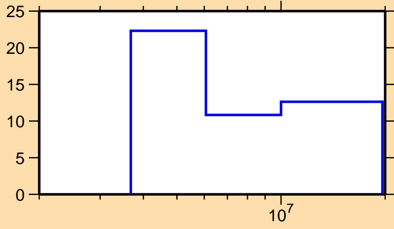
\Delta\sigma/\sigma vs. E for ^{144}\text{Pr}(n,2n)
