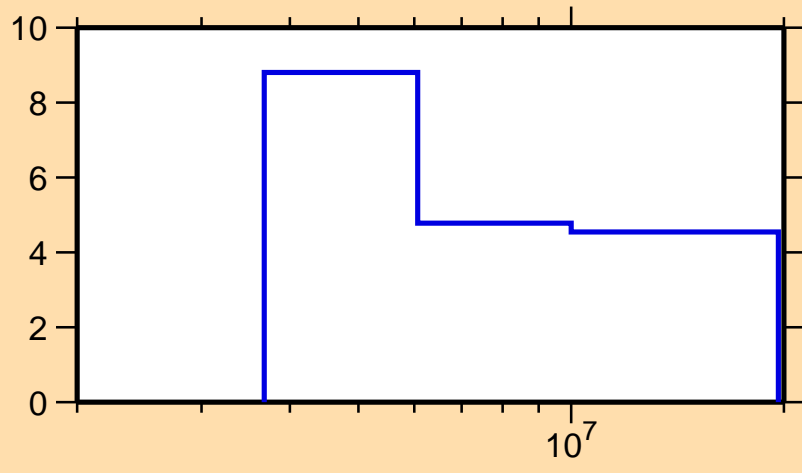
\Delta\sigma/\sigma vs. E for ^{144}\text{Pr}(n,\text{tot.})
