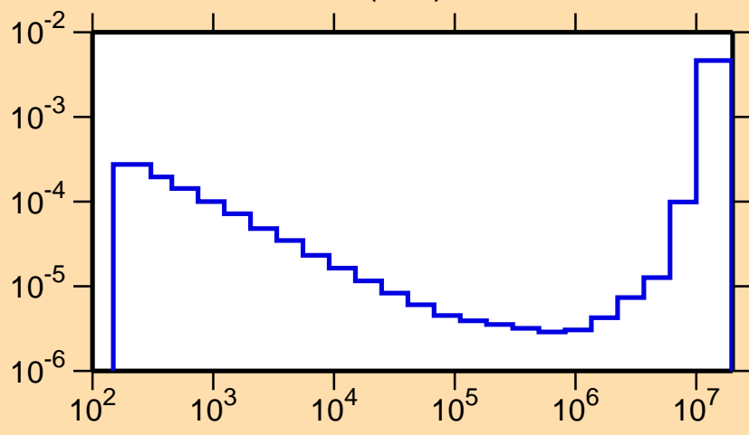
\sigma vs. E for ^{144}\text{Pr}(n,\alpha)
