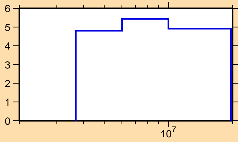
\Delta\sigma/\sigma vs. E for ^{144}\text{Pr}(n,\text{nonel.})
