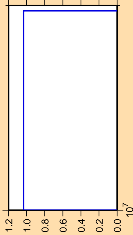
\Delta\sigma/\sigma vs. E for ^{144}\text{Pr}(\text{mt } 45)
