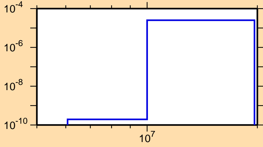
\sigma vs. E for ^{144}\text{Pr}(n,2n\alpha)
