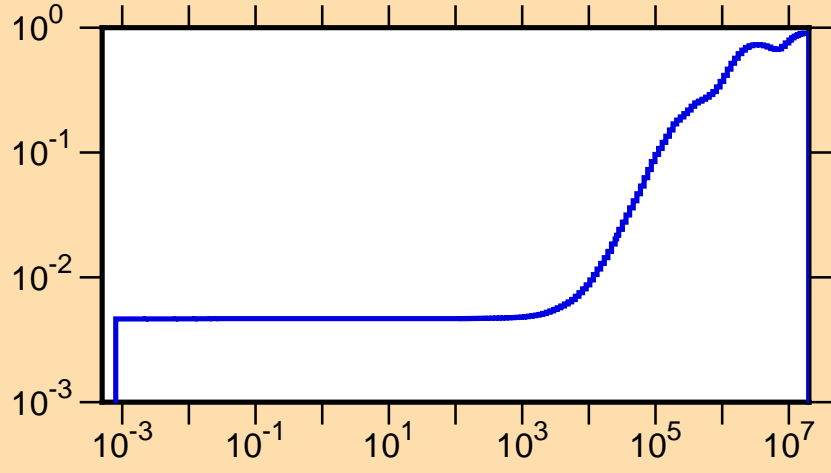
\mu vs. E for ^{145}\text{Pr}(\text{mt251})
