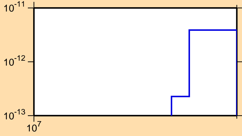
\sigma vs. E for ^{145}\text{Pr}(\text{mt } 45)
