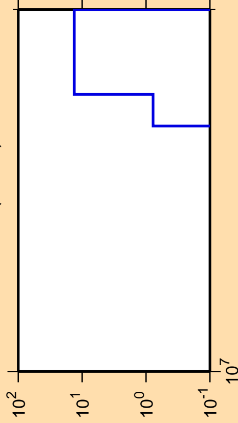
\Delta\sigma/\sigma vs. E for ^{145}\text{Pr}(\text{mt } 45)
