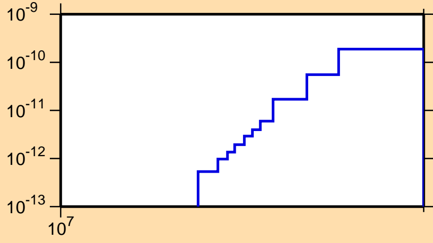
\sigma vs. E for ^{145}\text{Pr}(n,p\alpha)
