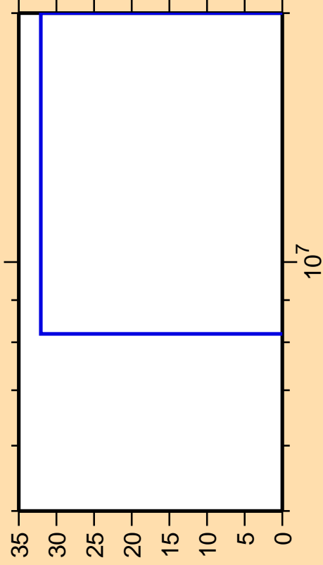
\Delta\sigma/\sigma vs. E for ^{145}\text{Pr}(n,3n)
