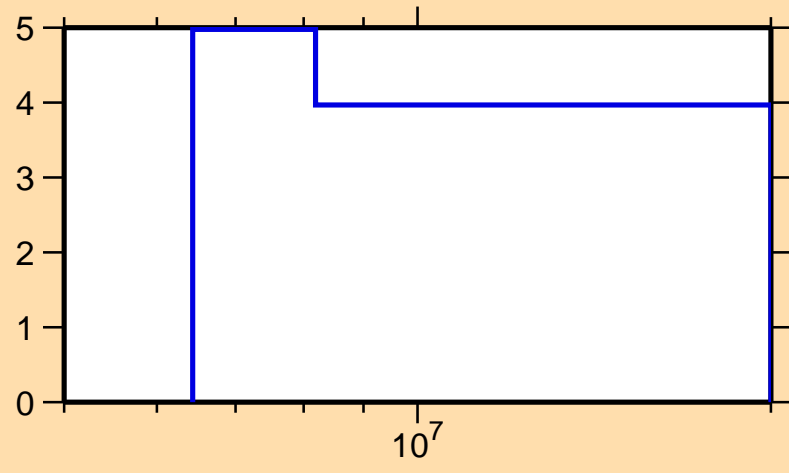
\Delta\sigma/\sigma vs. E for ^{145}\text{Pr}(n,\text{tot.})
