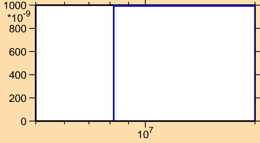
\sigma vs. E for ^{145}\text{Pr}(n,2n\alpha)
