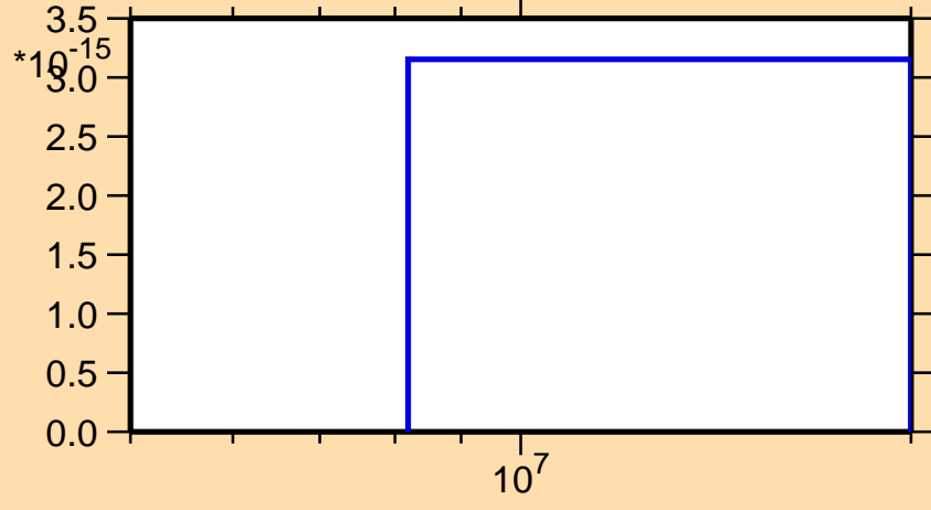
\sigma vs. E for ^{145}\text{Pr}(\text{mt } 11)
