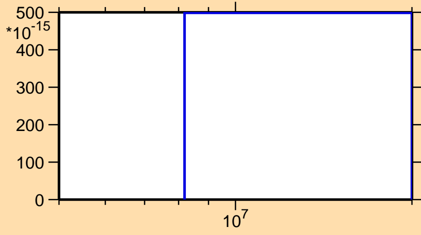
\sigma vs. E for ^{145}\text{Pr}(\text{mt117})
