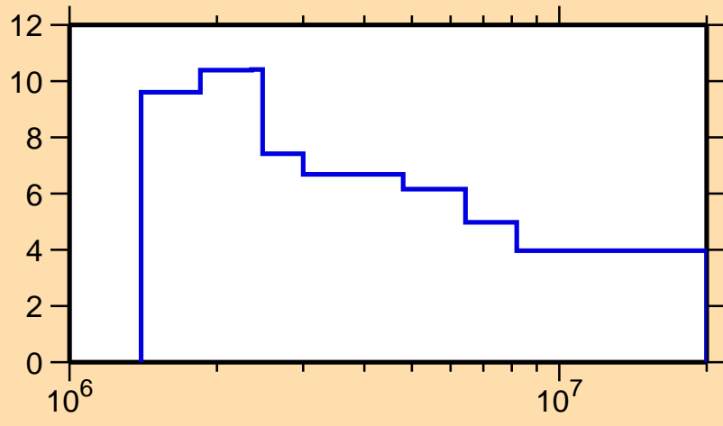
\Delta\sigma/\sigma vs. E for ^{145}\text{Pr}(n,\text{tot.})
