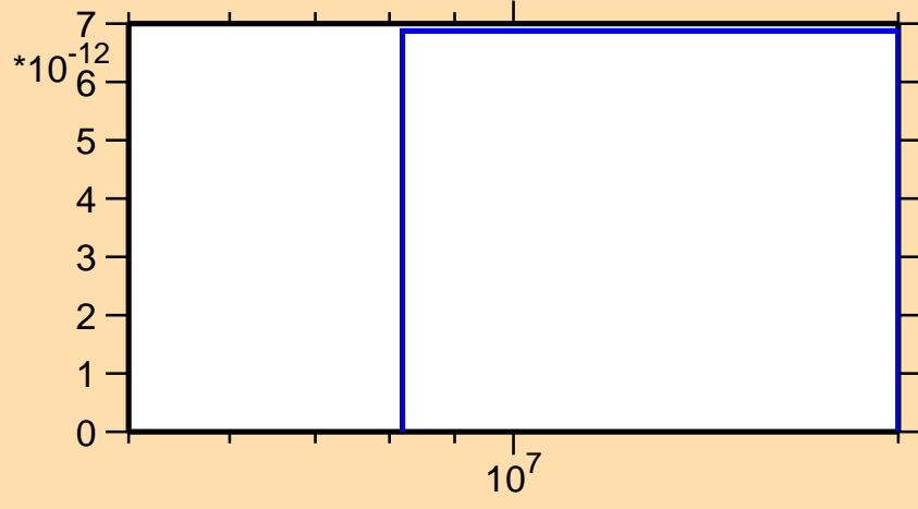
\sigma vs. E for ^{145}\text{Pr}(n,p\alpha)
