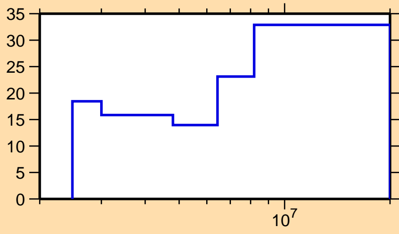
\Delta\sigma/\sigma vs. E for ^{145}\text{Pr}(n,n\text{cont.})
