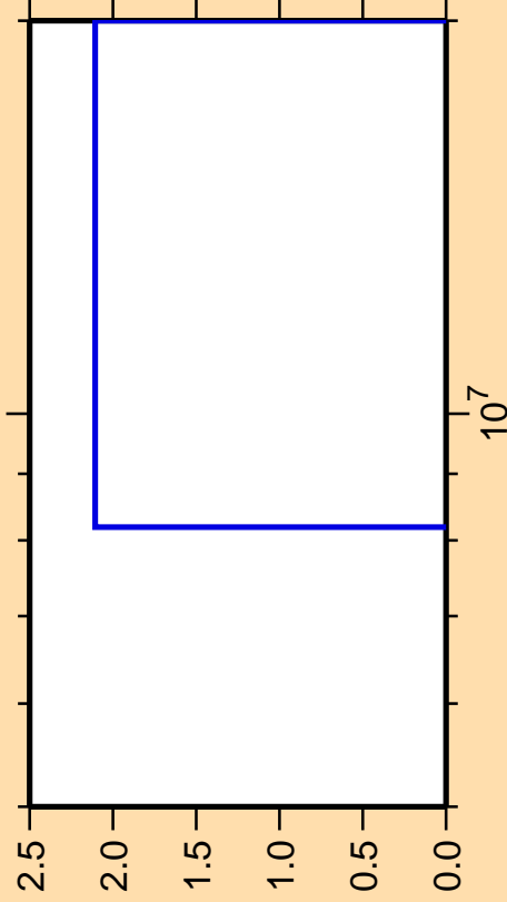
\Delta\sigma/\sigma vs. E for ^{145}\text{Pr}(\text{mt117})
