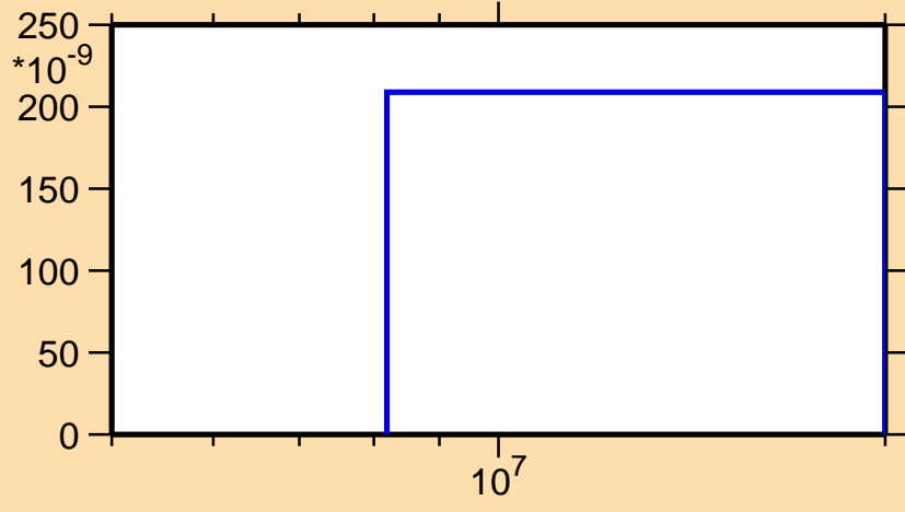
\sigma vs. E for ^{145}\text{Pr}(n,\text{nd})
