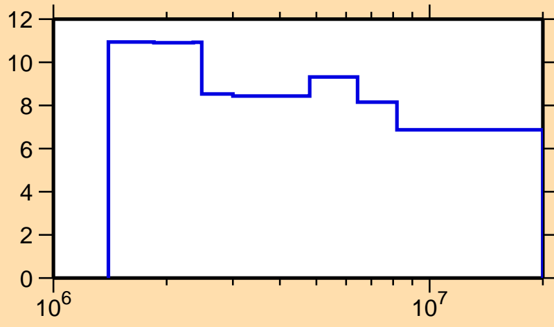
\Delta\sigma/\sigma vs. E for ^{145}\text{Pr}(n,\text{nonel.})
