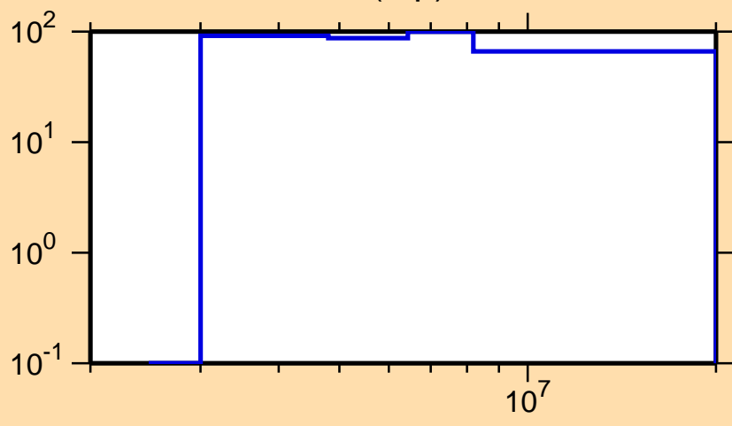
\Delta\sigma/\sigma vs. E for ^{145}\text{Pr}(n,p)
