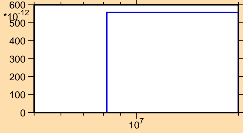
\sigma vs. E for ^{145}\text{Pr}(n,3n\alpha)
