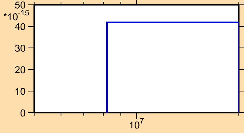
\sigma vs. E for ^{145}\text{Pr}(\text{mt } 45)
