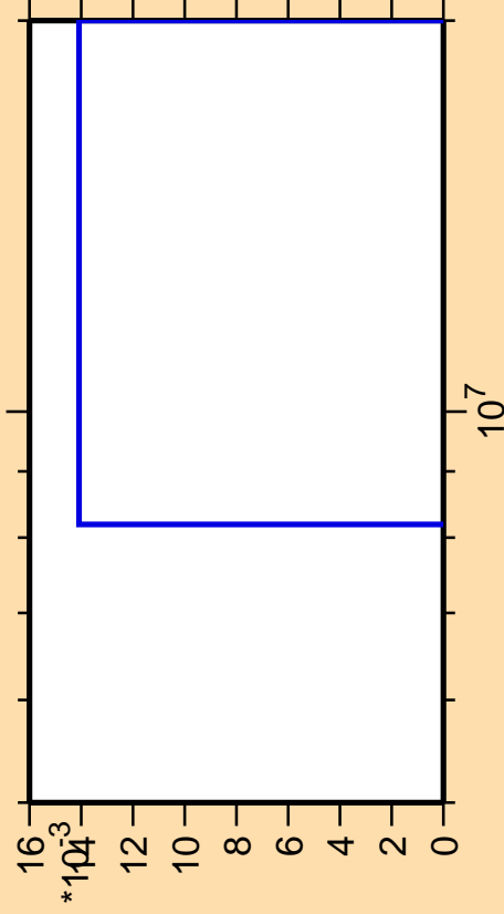
\Delta\sigma/\sigma vs. E for ^{145}\text{Pr}(\text{mt } 11)
