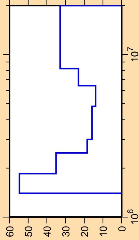
\Delta\sigma/\sigma vs. E for ^{145}\text{Pr}(n,n\text{cont.})
