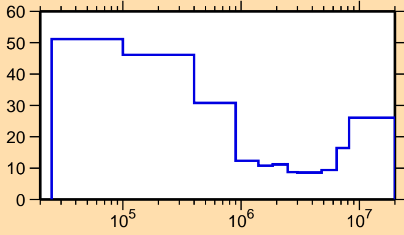
\Delta\sigma/\sigma vs. E for ^{145}\text{Pr}(n,\text{inel.})
