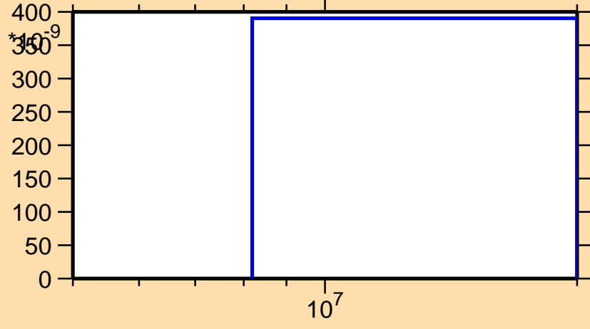
\sigma vs. E for ^{145}\text{Pr}(n,nt)
