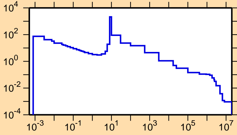
\sigma vs. E for ^{145}\text{Pr}(n,\gamma)
