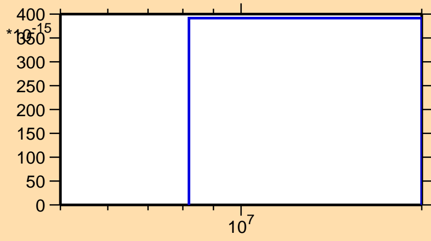
\sigma vs. E for ^{145}\text{Pr}(n,\text{He3})
