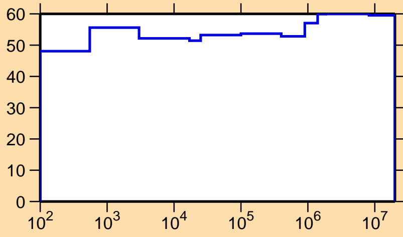
\Delta\sigma/\sigma vs. E for ^{145}\text{Pr}(n,\gamma)
