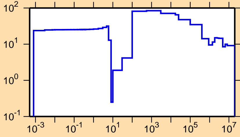
\Delta\sigma/\sigma vs. E for ^{145}\text{Pr}(n,\text{el.})
