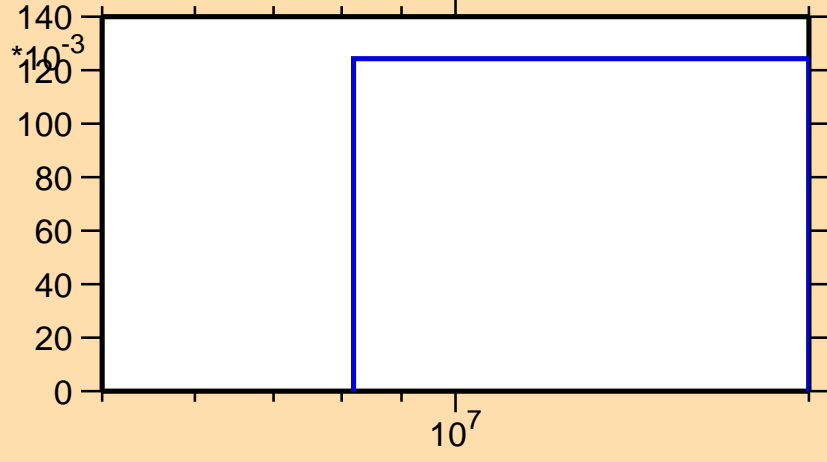
\sigma vs. E for ^{145}\text{Pr}(n,3n)
