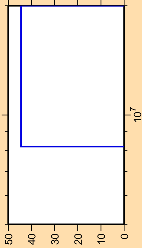
\Delta\sigma/\sigma vs. E for ^{145}\text{Pr}(n,p\alpha)
