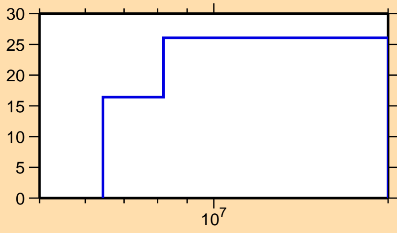
\Delta\sigma/\sigma vs. E for ^{145}\text{Pr}(n,\text{inel.})
