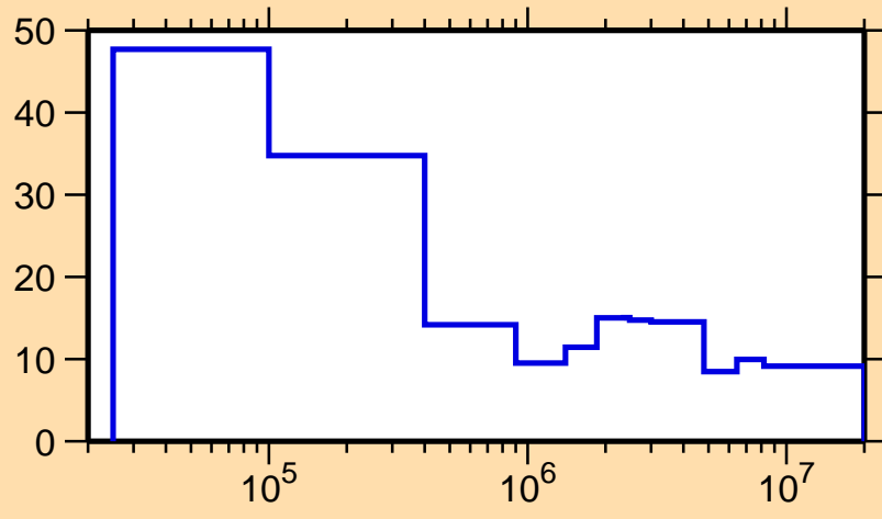
\Delta\sigma/\sigma vs. E for ^{145}\text{Pr}(n,\text{el.})
