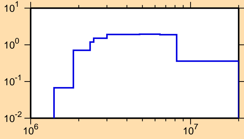
\sigma vs. E for ^{145}\text{Pr}(n,n\text{cont.})
