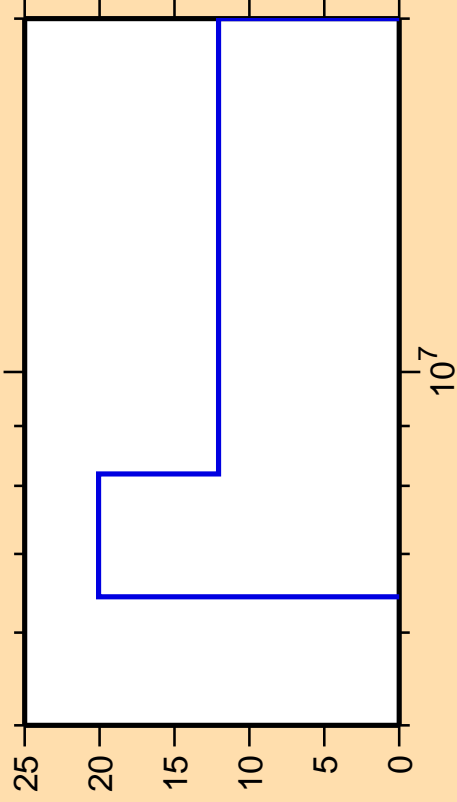
\Delta\sigma/\sigma vs. E for ^{145}\text{Pr}(n,2n)
