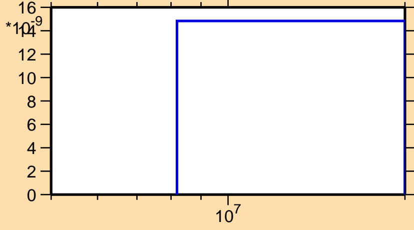
\sigma vs. E for ^{145}\text{Pr}(n,2np)
