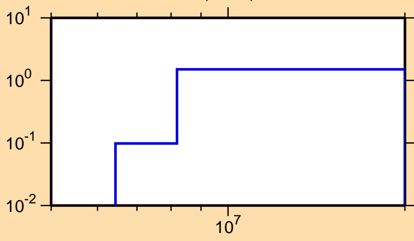
\sigma vs. E for ^{145}\text{Pr}(n,2n)
