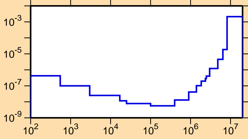
\sigma vs. E for ^{145}\text{Pr}(n,\alpha)
