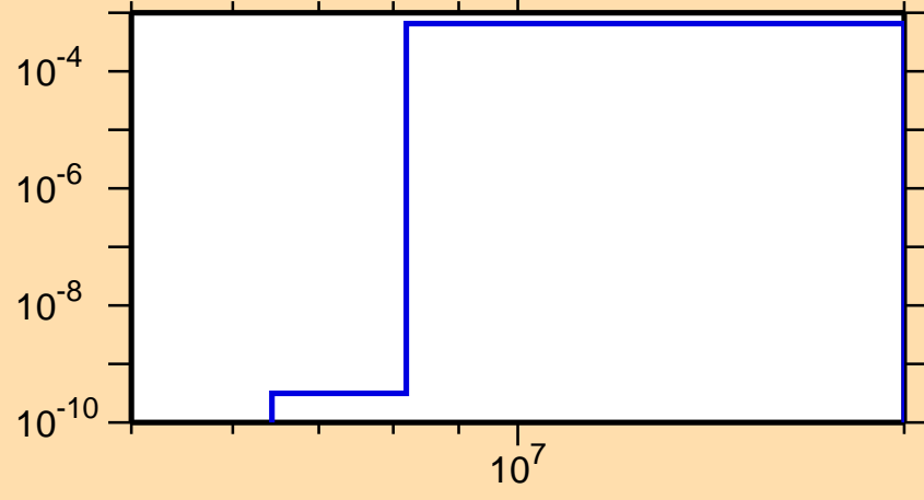
\sigma vs. E for ^{145}\text{Pr}(n,d)
