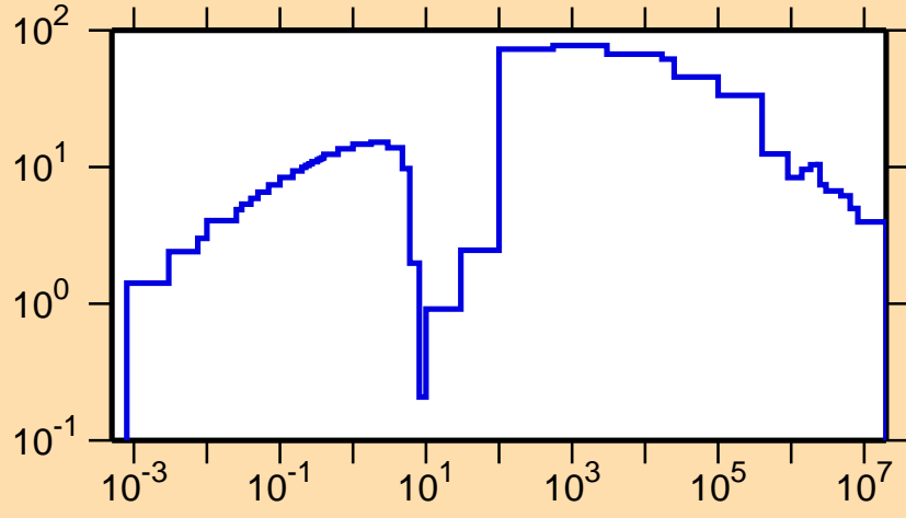
\Delta\sigma/\sigma vs. E for ^{145}\text{Pr}(n,\text{tot.})
