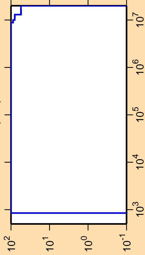
\Delta\sigma/\sigma vs. E for ^{146}\text{Pr}(n,\alpha)
