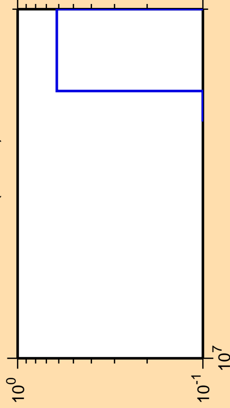
\Delta\sigma/\sigma vs. E for ^{146}\text{Pr}(\text{mt } 45)
