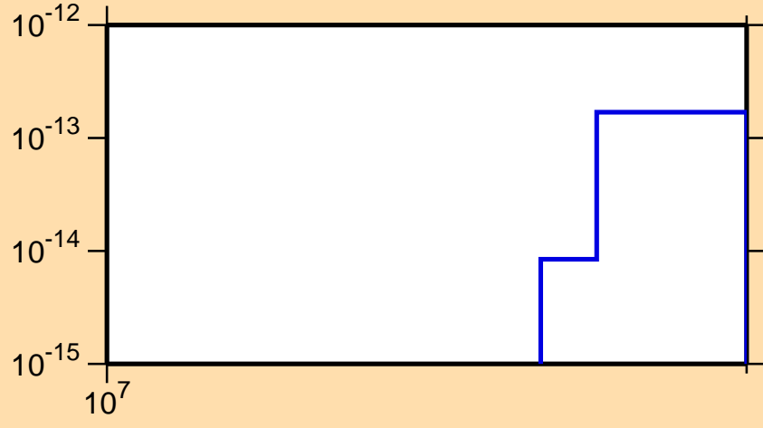
\sigma vs. E for ^{146}\text{Pr}(\text{mt } 45)
