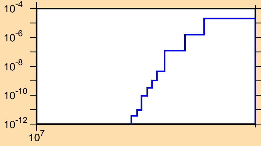
\sigma vs. E for ^{146}\text{Pr}(n,2np)
