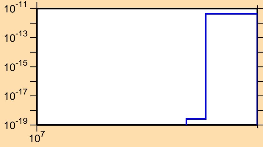
\sigma vs. E for ^{146}\text{Pr}(\text{mt 11})
