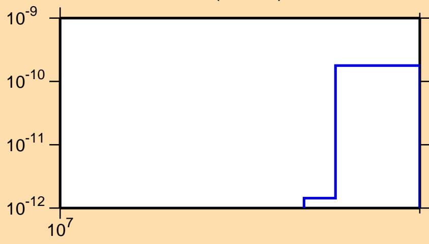
\sigma vs. E for ^{146}\text{Pr}(n,\text{He3})
