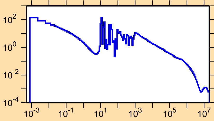
\sigma vs. E for ^{146}\text{Pr}(n,\gamma)
