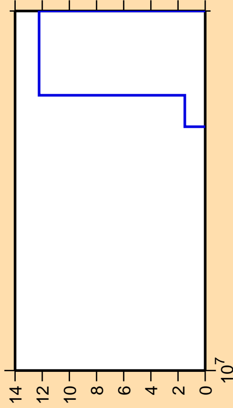
\Delta\sigma/\sigma vs. E for ^{146}\text{Pr}(\text{mt117})
