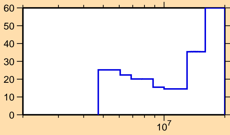
\Delta\sigma/\sigma vs. E for ^{146}\text{Pr}(n,2n)
