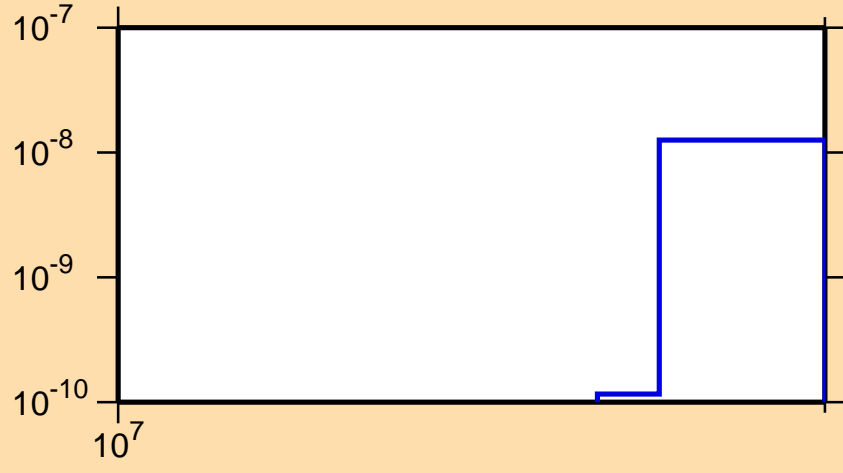
\sigma vs. E for ^{146}\text{Pr}(n,3n\alpha)
