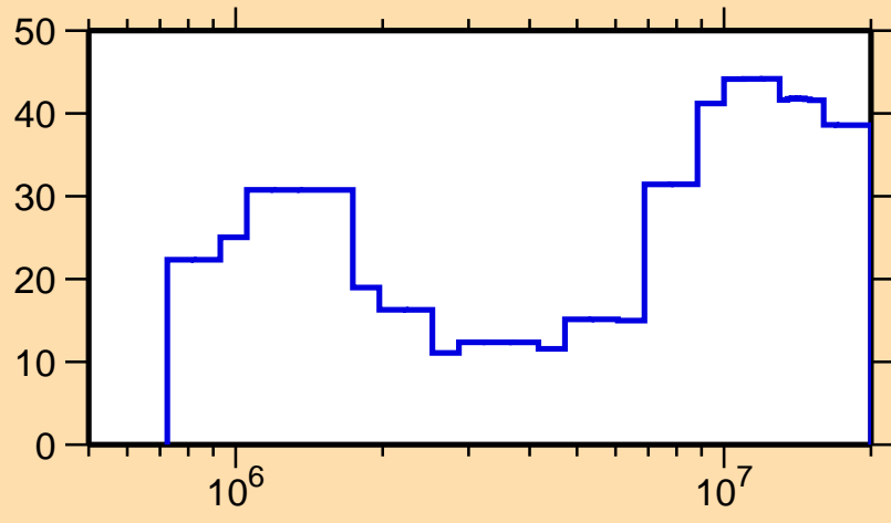
\Delta\sigma/\sigma vs. E for ^{146}\text{Pr}(n,\text{inel.})
