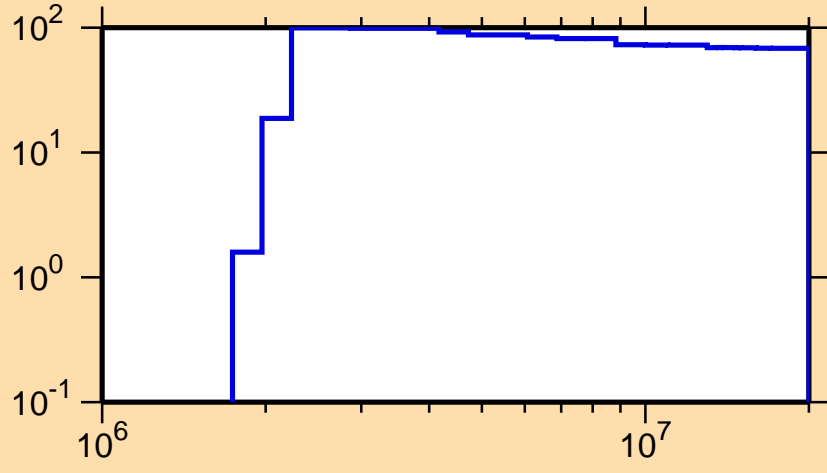
\Delta\sigma/\sigma vs. E for ^{146}\text{Pr}(n,p)
