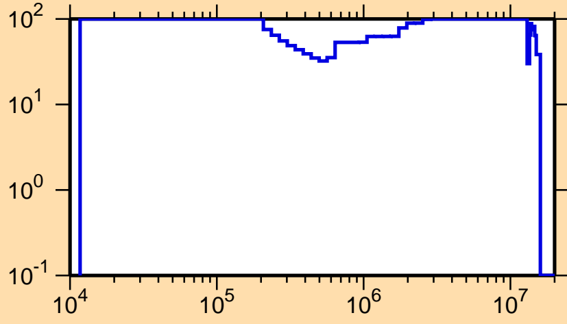
\Delta\sigma/\sigma vs. E for ^{146}\text{Pr}(n,n_1)
