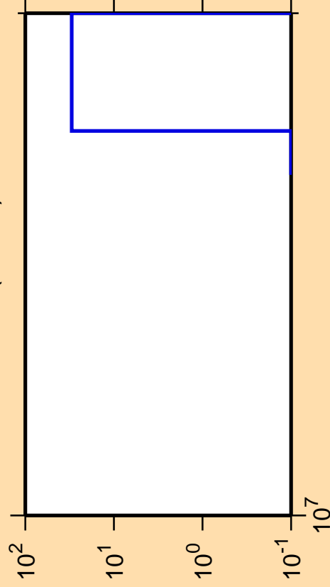
\Delta\sigma/\sigma vs. E for ^{146}\text{Pr}(\text{mt 11})
