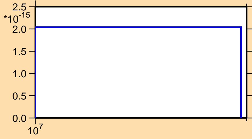
\sigma vs. E for ^{146}\text{Pr}(\text{mt } 45)
