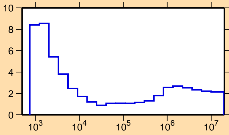
\sigma vs. E for ^{146}\text{Pr}(n,\text{nonel.})
