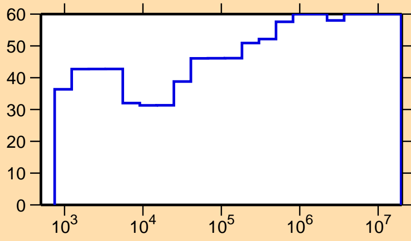
\Delta\sigma/\sigma vs. E for ^{146}\text{Pr}(n,\gamma)
