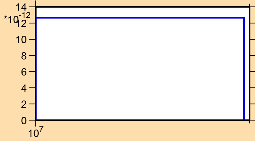
\sigma vs. E for ^{146}\text{Pr}(n,p\alpha)
