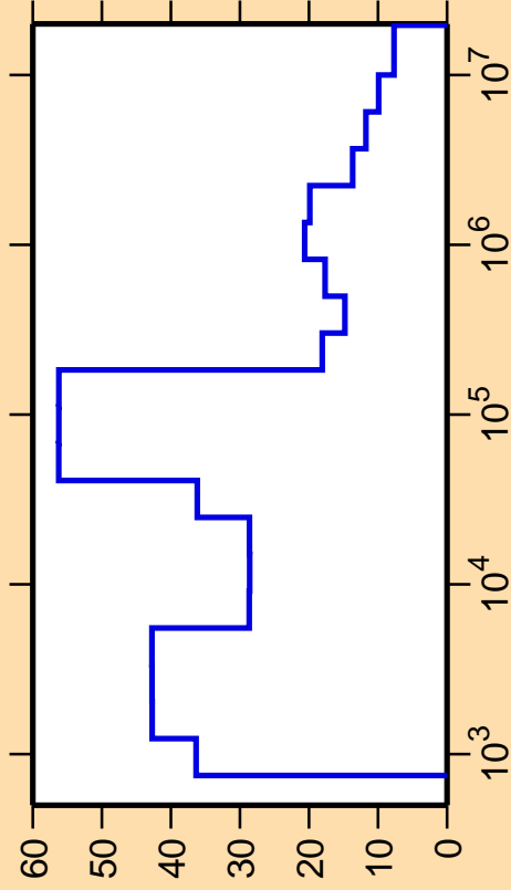
\Delta\sigma/\sigma vs. E for ^{146}\text{Pr}(n,\text{nonel.})
