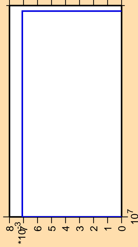
\Delta\sigma/\sigma vs. E for ^{146}\text{Pr}(\text{mt } 45)
