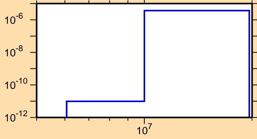
\sigma vs. E for ^{146}\text{Pr}(n,2n\alpha)
