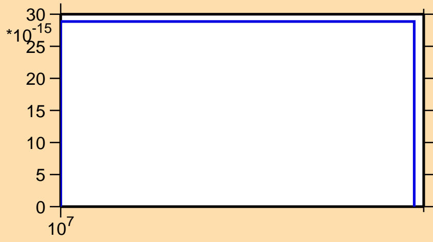
\sigma vs. E for ^{146}\text{Pr}(\text{mt117})
