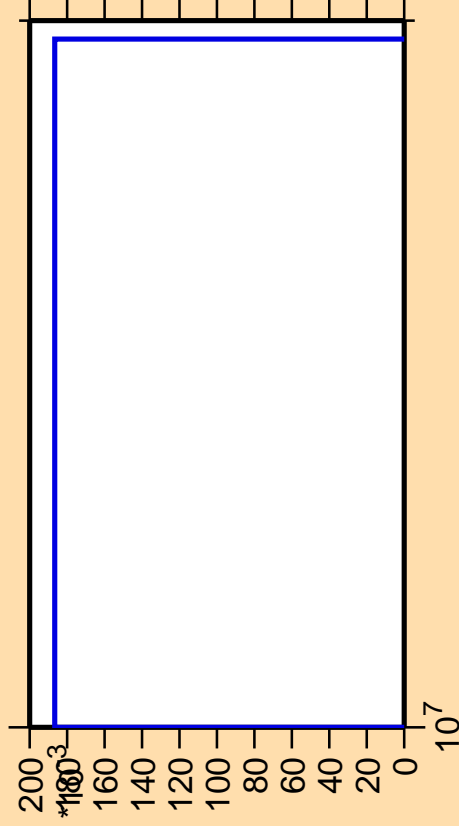
\Delta\sigma/\sigma vs. E for ^{146}\text{Pr}(\text{mt117})
