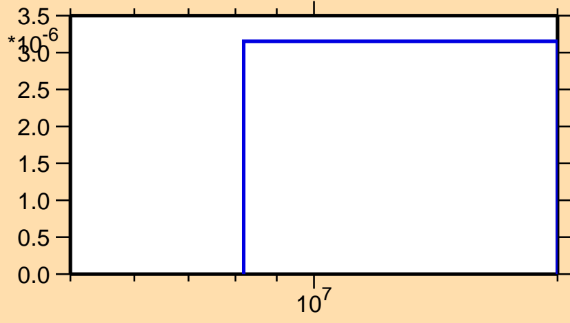
\sigma vs. E for ^{146}\text{Pr}(n,\text{nd})
