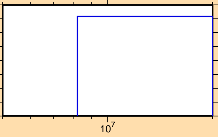
\sigma vs. E for ^{146}\text{Pr}(\text{mt } 11)
