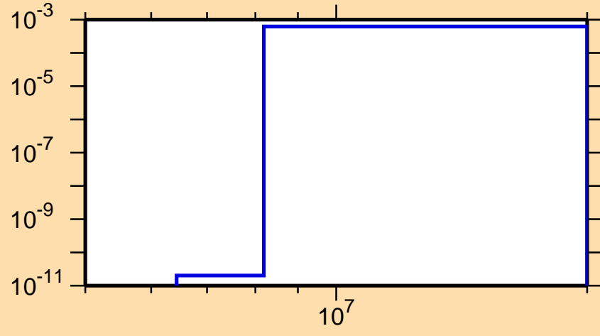
\sigma vs. E for ^{146}\text{Pr}(n,d)
