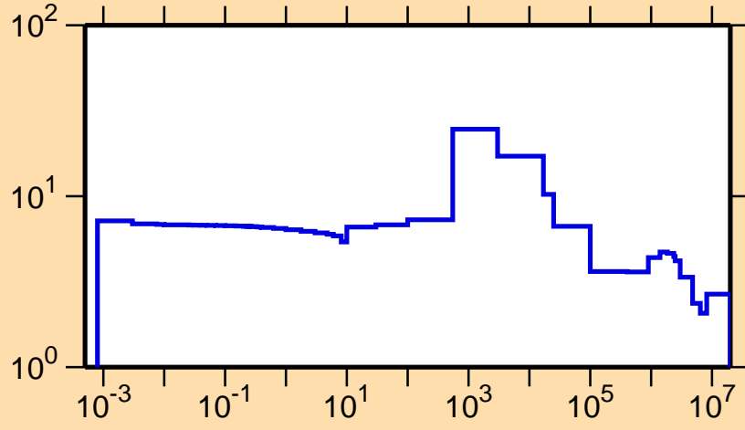
\sigma vs. E for ^{146}\text{Pr}(n,\text{el.})
