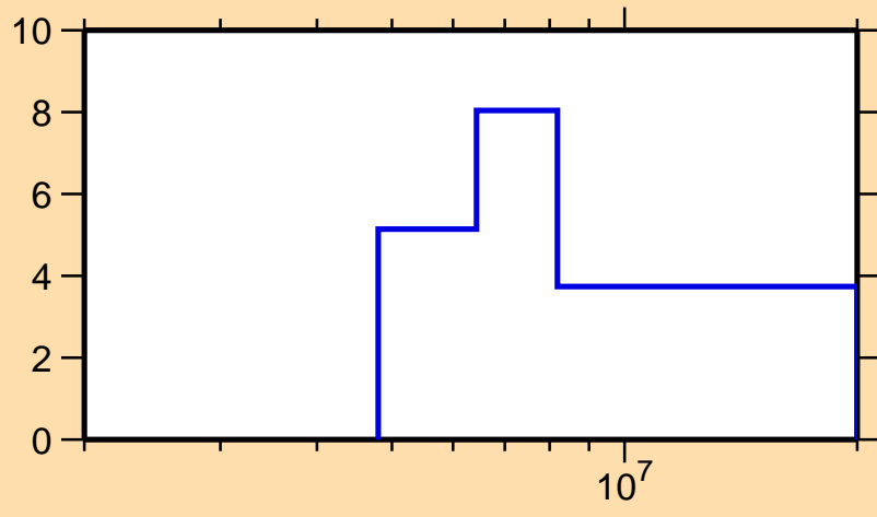
\Delta\sigma/\sigma vs. E for ^{146}\text{Pr}(n,\text{tot.})
