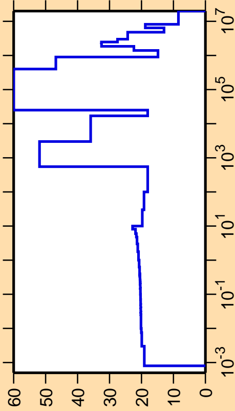
\Delta\sigma/\sigma vs. E for ^{146}\text{Pr}(n,\text{el.})
