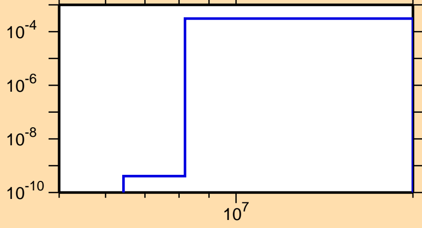
\sigma vs. E for ^{146}\text{Pr}(n,t)
