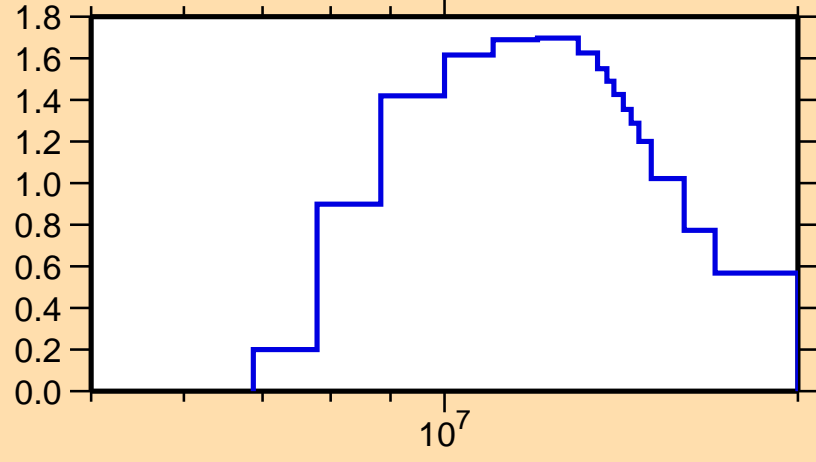
\sigma vs. E for ^{147}\text{Pr}(n,2n)
