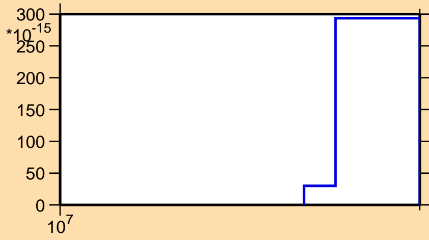
\sigma vs. E for ^{147}\text{Pr}(\text{mt117})
