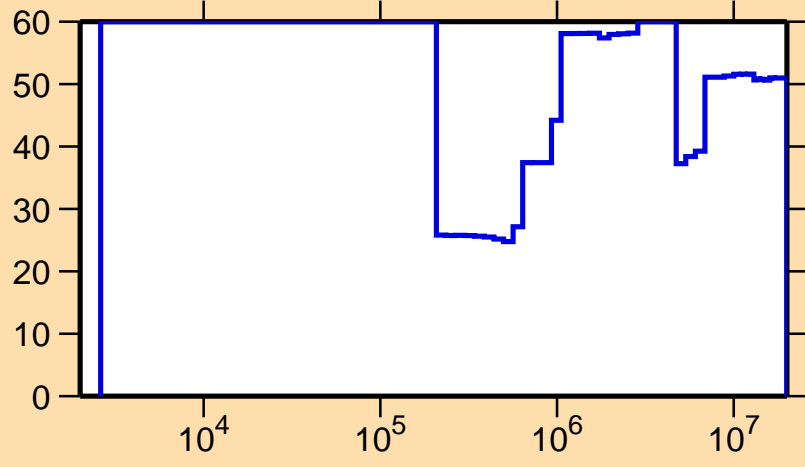
\Delta\sigma/\sigma vs. E for ^{147}\text{Pr}(n,n_1)
