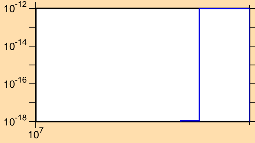
\sigma vs. E for ^{147}\text{Pr}(\text{mt 11})
