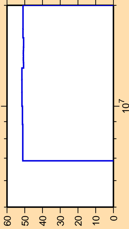
\Delta\sigma/\sigma vs. E for ^{147}\text{Pr}(n,n_1)
