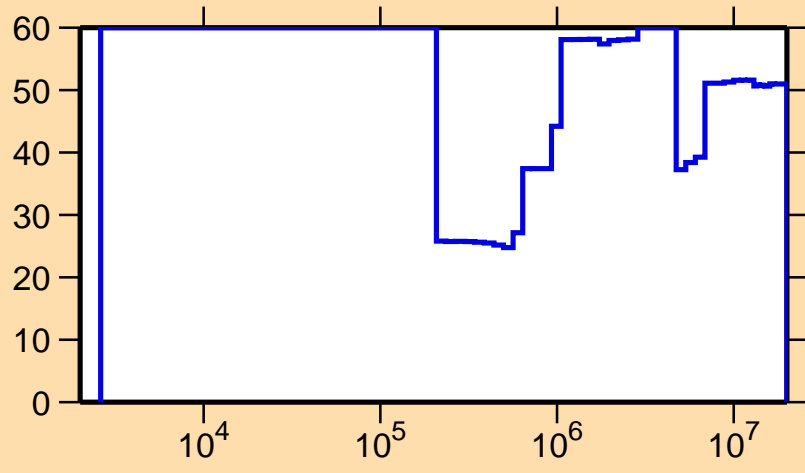
\Delta\sigma/\sigma vs. E for ^{147}\text{Pr}(n,n_1)
