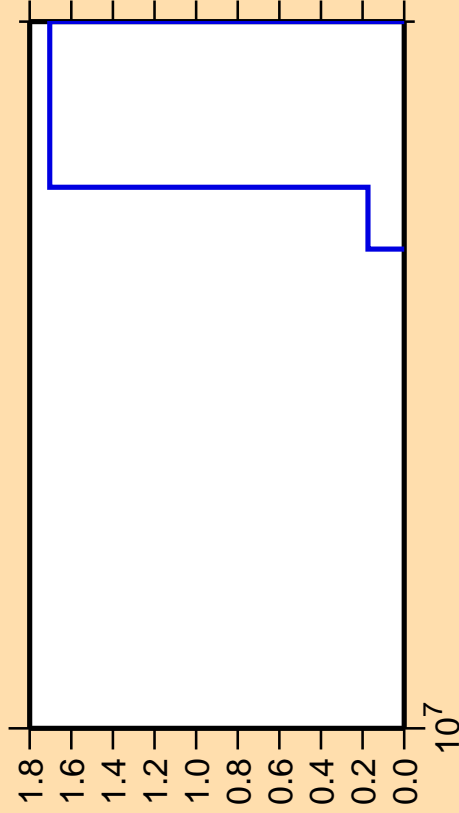
\Delta\sigma/\sigma vs. E for ^{147}\text{Pr}(\text{mt117})
