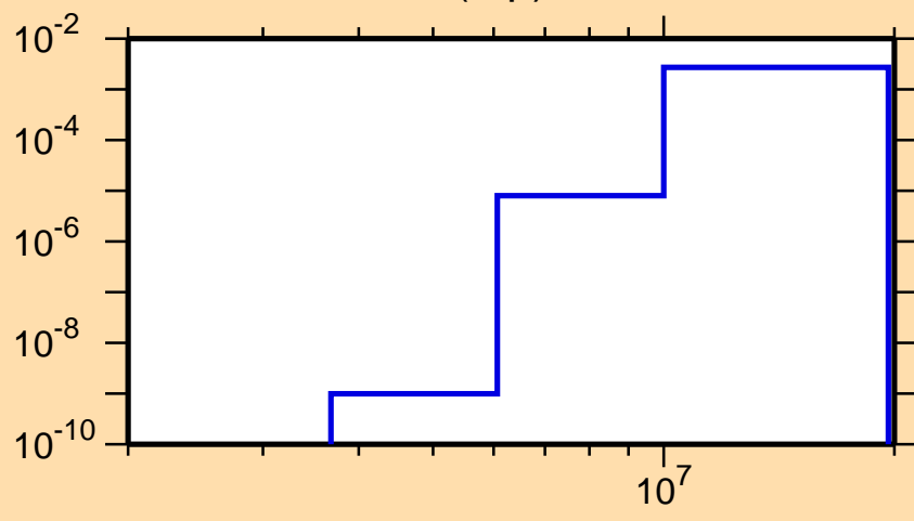
\sigma vs. E for ^{147}\text{Pr}(n,p)
