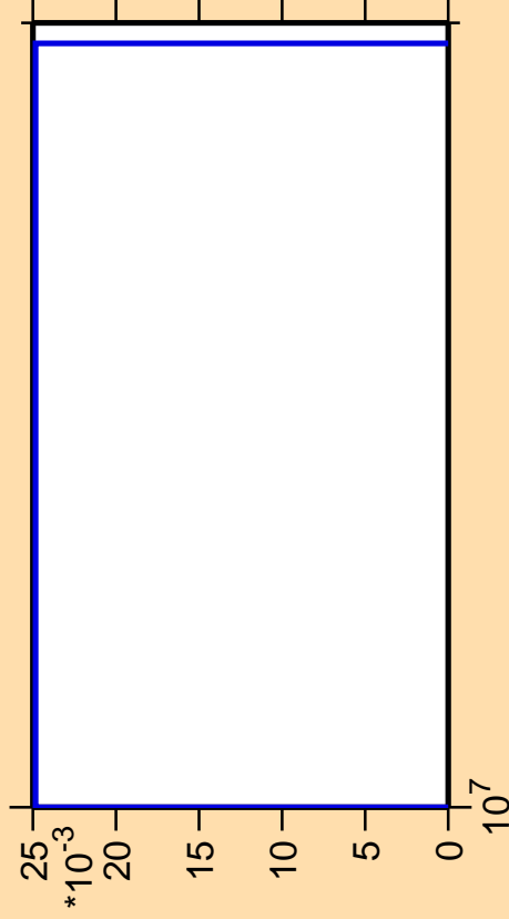
\Delta\sigma/\sigma vs. E for ^{147}\text{Pr}(\text{mt117})
