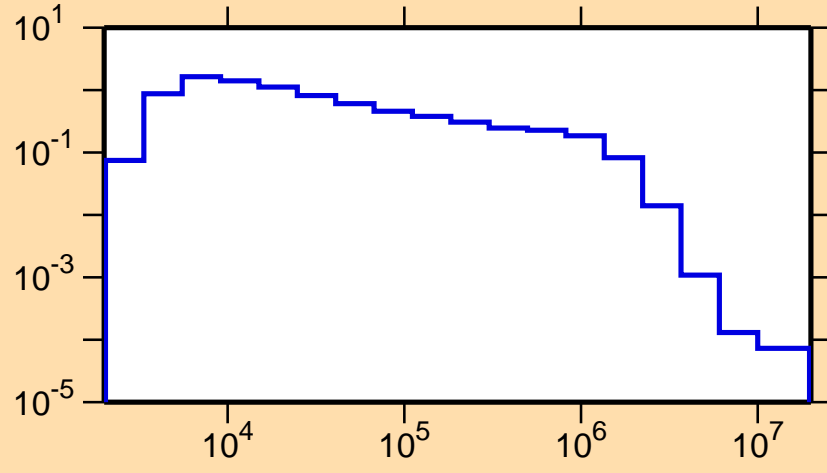
\sigma vs. E for ^{147}\text{Pr}(n,n_1)
