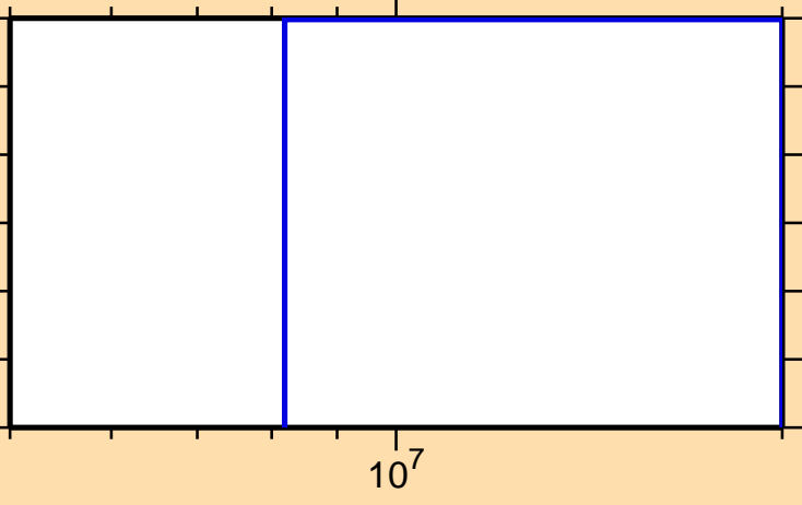
\sigma vs. E for ^{147}\text{Pr}(n,nt)
