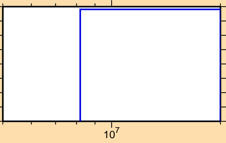
\sigma vs. E for ^{147}\text{Pr}(\text{mt117})
