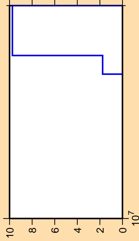
\Delta\sigma/\sigma vs. E for ^{148}\text{Pr}(n,p\alpha)
