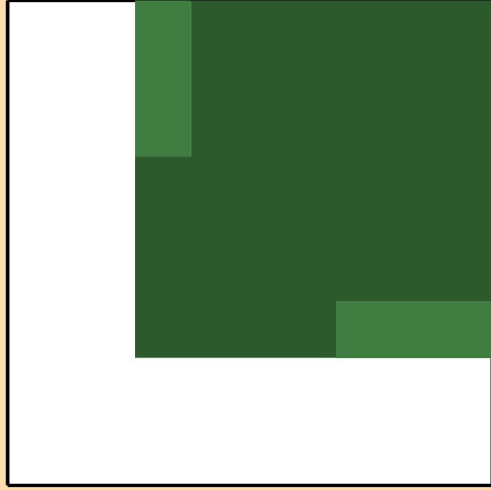
\sigma vs. E for ^{148}\text{Pr}(n,3n)
