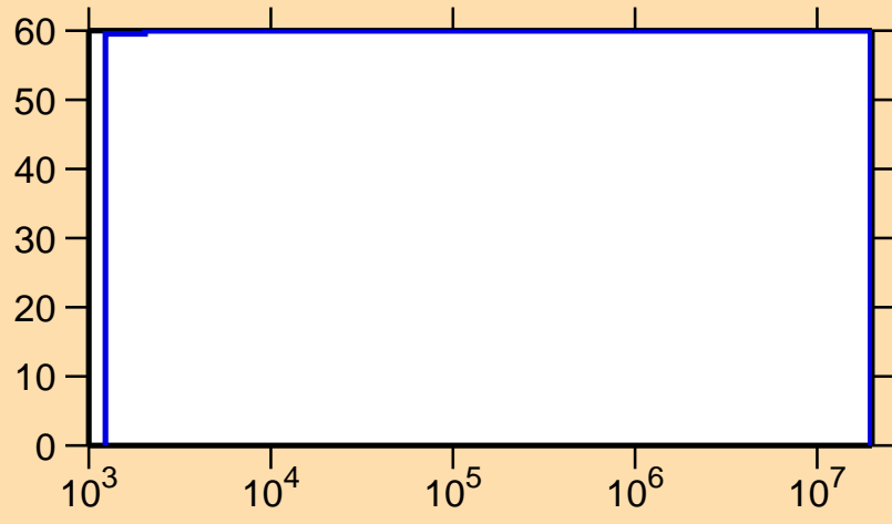
\Delta\sigma/\sigma vs. E for ^{148}\text{Pr}(n,\gamma)
