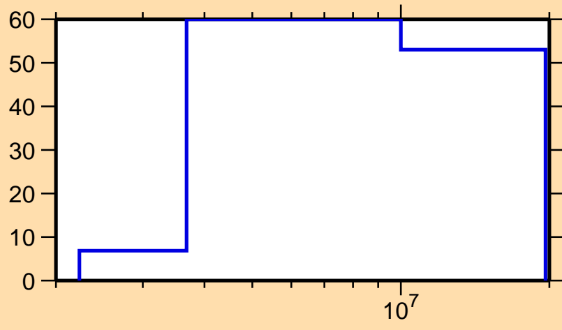
\Delta\sigma/\sigma vs. E for ^{148}\text{Pr}(n,p)
