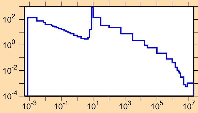
\sigma vs. E for ^{148}\text{Pr}(n,\gamma)
