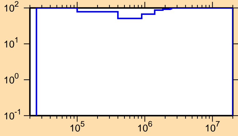
\Delta\sigma/\sigma vs. E for ^{148}\text{Pr}(n,n_1)
