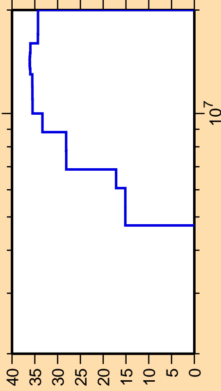
\Delta\sigma/\sigma vs. E for ^{148}\text{Pr}(n,n\text{cont.})
