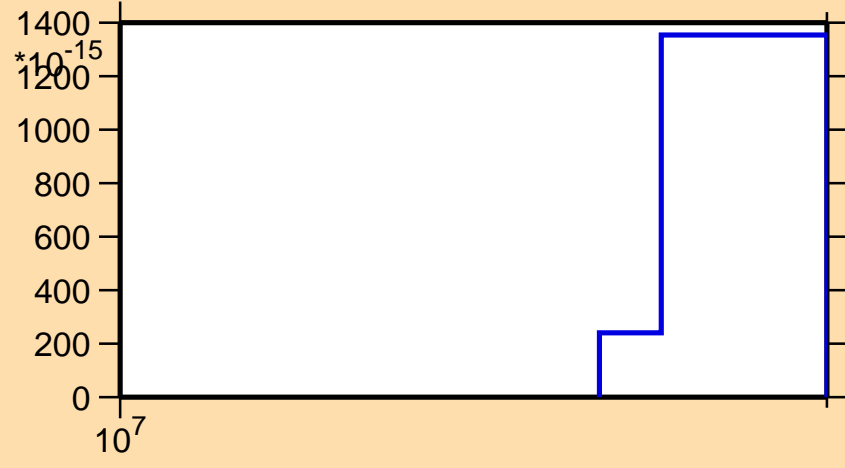
\sigma vs. E for ^{148}\text{Pr}(n,p\alpha)
