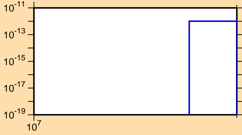
\sigma vs. E for ^{148}\text{Pr}(\text{mt 11})
