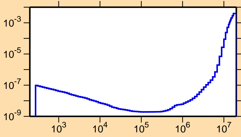
\sigma vs. E for ^{148}\text{Pr}(n,\alpha)
