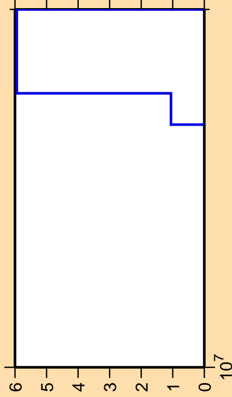
\Delta\sigma/\sigma vs. E for ^{148}\text{Pr}(n,p\alpha)
