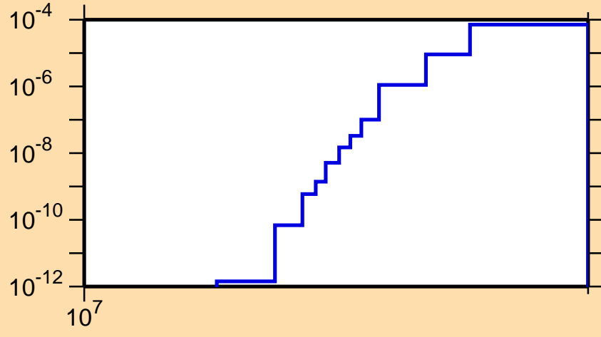
\sigma vs. E for ^{148}\text{Pr}(n,\text{nd})
