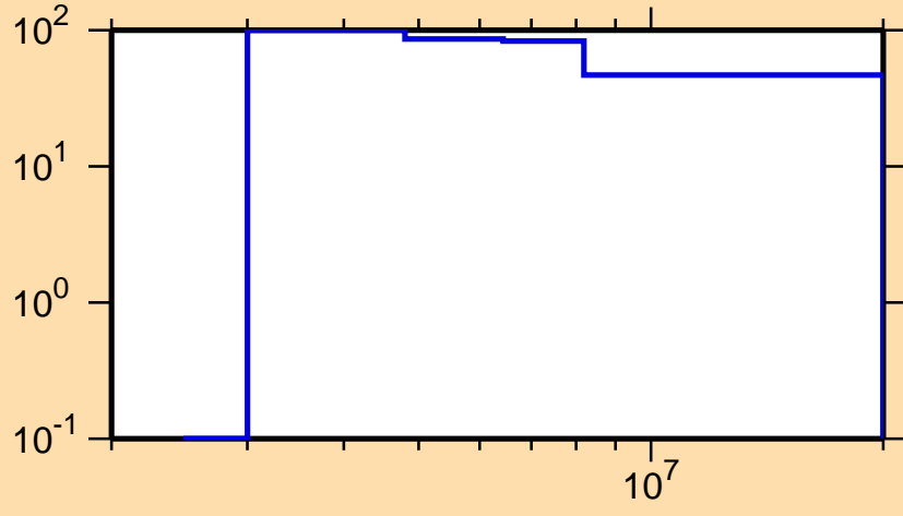
\Delta\sigma/\sigma vs. E for ^{148}\text{Pr}(n,p)
