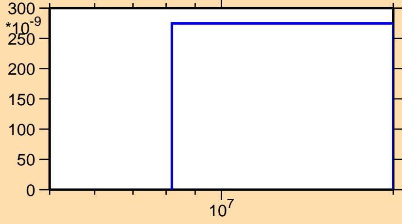
\sigma vs. E for ^{148}\text{Pr}(n,2n\alpha)
