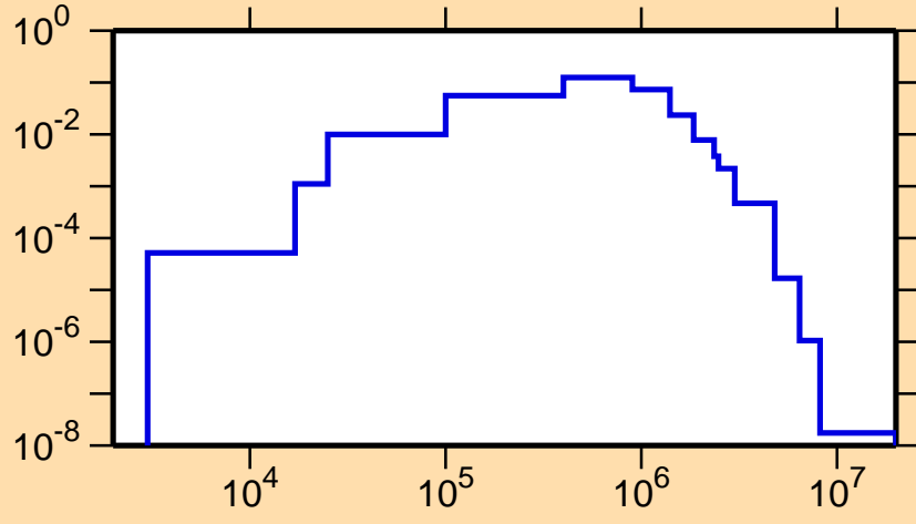
\sigma vs. E for ^{148}\text{Pr}(n,n_3)
