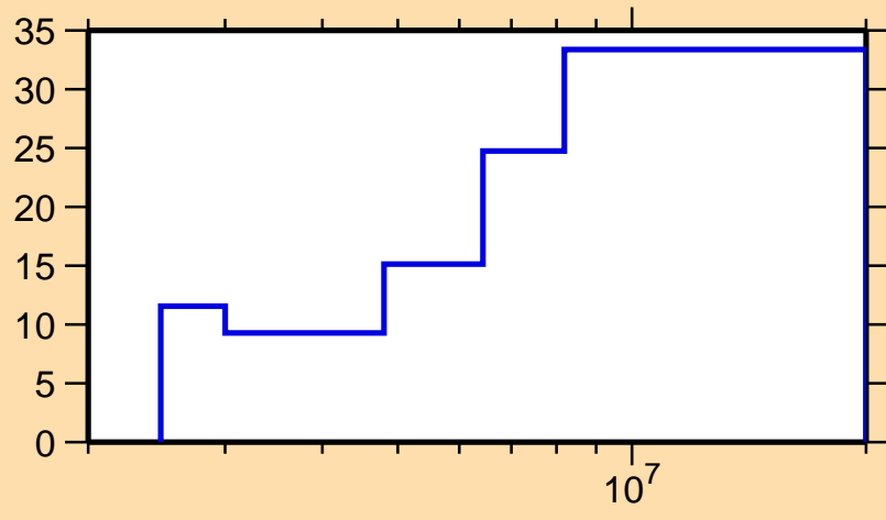
\Delta\sigma/\sigma vs. E for ^{148}\text{Pr}(n,n\text{cont.})
