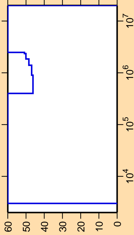
\Delta\sigma/\sigma vs. E for ^{148}\text{Pr}(n,n_3)
