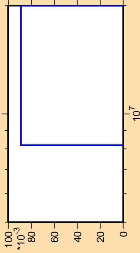
\Delta\sigma/\sigma vs. E for ^{148}\text{Pr}(n,p\alpha)
