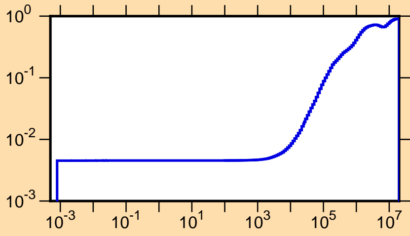
\mu vs. E for ^{149}\text{Pr}(\text{mt251})
