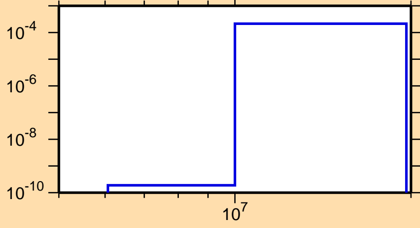
\sigma vs. E for ^{149}\text{Pr}(n,d)
