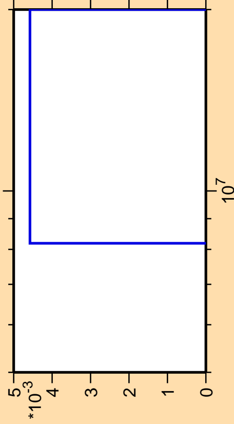
\Delta\sigma/\sigma vs. E for ^{149}\text{Pr}(\text{mt } 11)
