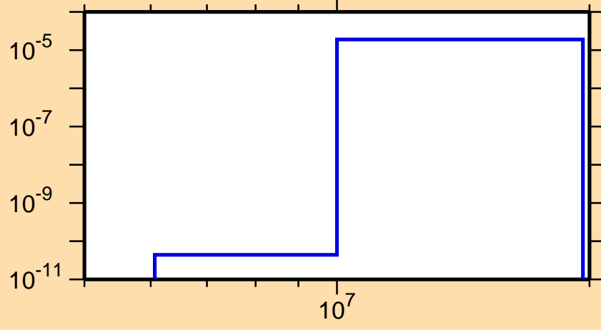
\sigma vs. E for ^{150}\text{Pr}(n,n\alpha)
