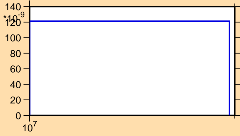
\sigma vs. E for ^{150}\text{Pr}(n,nt)
