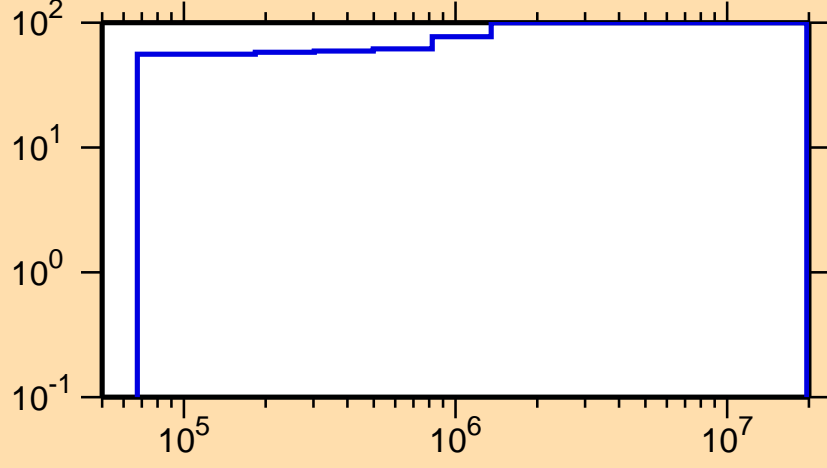
\Delta\sigma/\sigma vs. E for ^{150}\text{Pr}(n,n_1)
