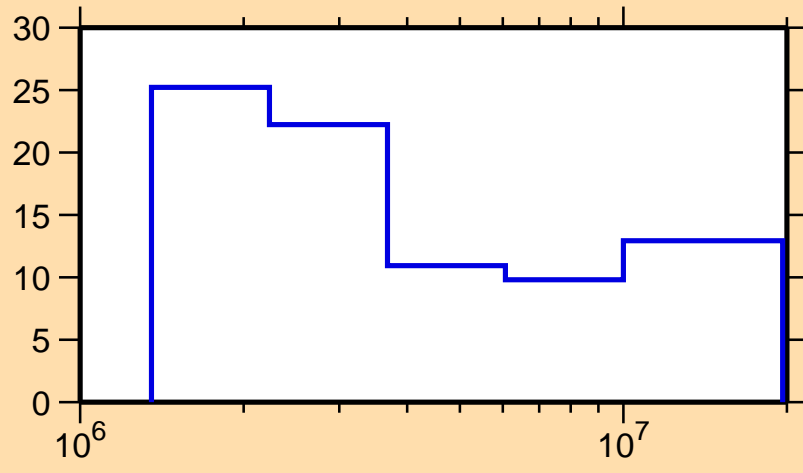
\Delta\sigma/\sigma vs. E for ^{150}\text{Pr}(n,\text{tot.})
