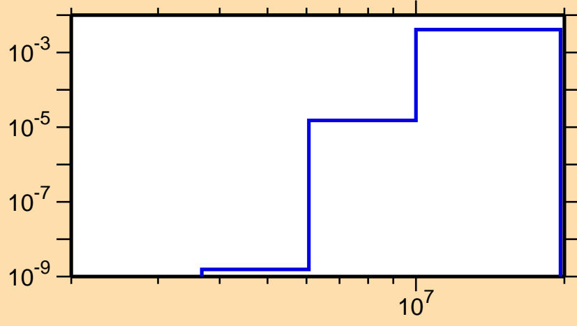
\sigma vs. E for ^{150}\text{Pr}(n,p)
