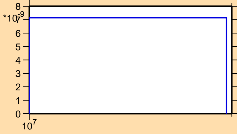
\sigma vs. E for ^{150}\text{Pr}(n,2np)
