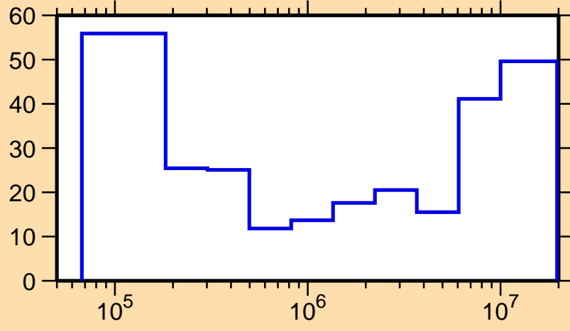
\Delta\sigma/\sigma vs. E for ^{150}\text{Pr}(n,\text{inel.})
