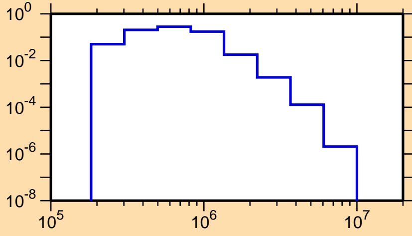
\sigma vs. E for ^{150}\text{Pr}(n,n_2)
