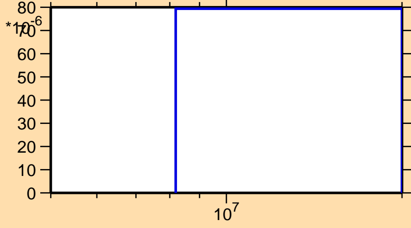
\sigma vs. E for ^{150}\text{Pr}(n,d)
