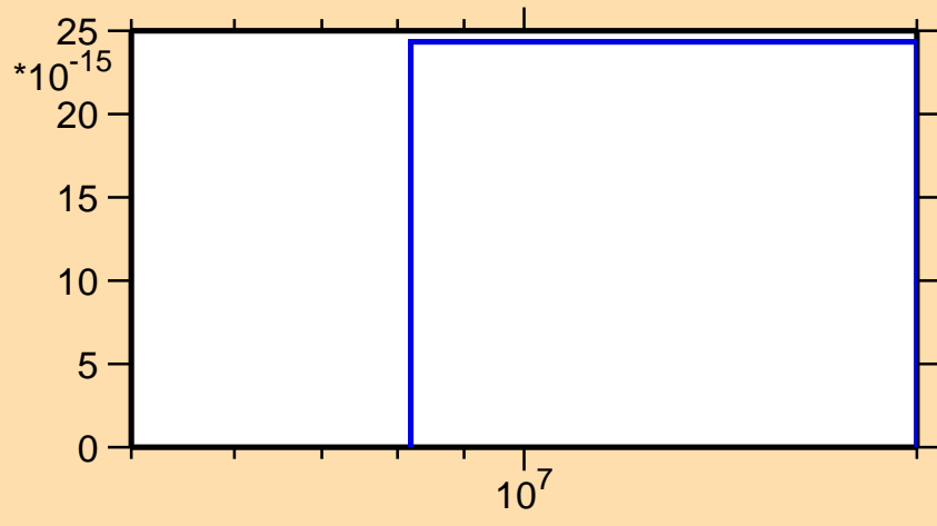
\sigma vs. E for ^{150}\text{Pr}(n,3n\alpha)
