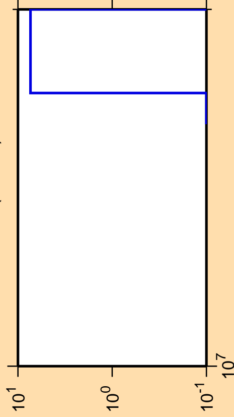
\Delta\sigma/\sigma vs. E for ^{151}\text{Pr}(n,3n\alpha)
