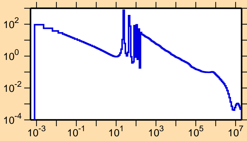
\sigma vs. E for ^{151}\text{Pr}(n,\gamma)
