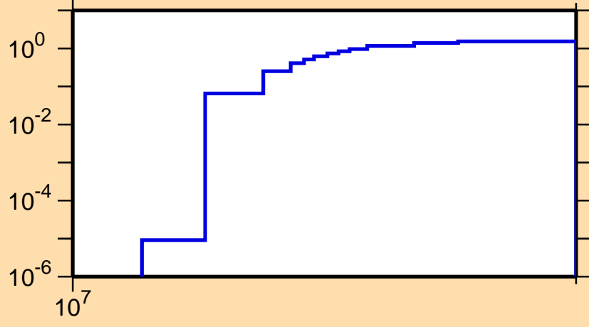
\sigma vs. E for ^{151}\text{Pr}(n,3n)
