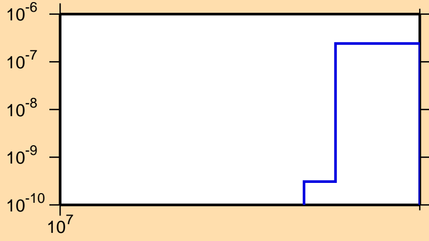
\sigma vs. E for ^{151}\text{Pr}(n,\text{nd})
