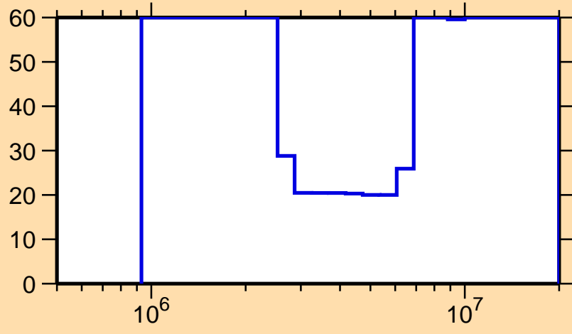
\Delta\sigma/\sigma vs. E for ^{151}\text{Pr}(n,n\text{cont.})
