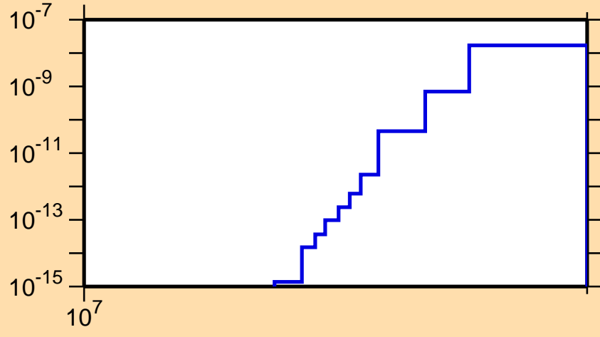
\sigma vs. E for ^{151}\text{Pr}(n,2n\alpha)
