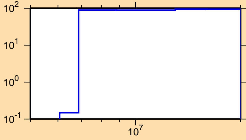
\Delta\sigma/\sigma vs. E for ^{151}\text{Pr}(n,p)
