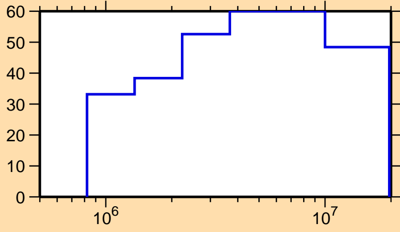
\Delta\sigma/\sigma vs. E for ^{151}\text{Pr}(n, el.)
