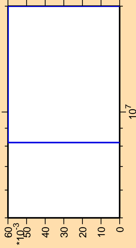
\Delta\sigma/\sigma vs. E for ^{151}\text{Pr}(n,3n\alpha)
