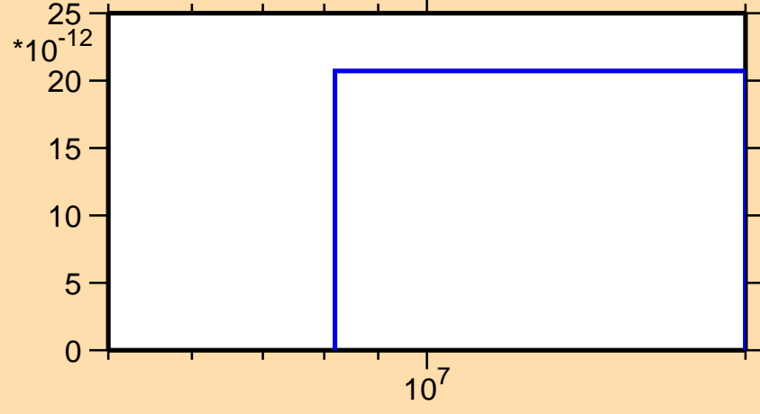
\sigma vs. E for ^{151}\text{Pr}(n,2np)
