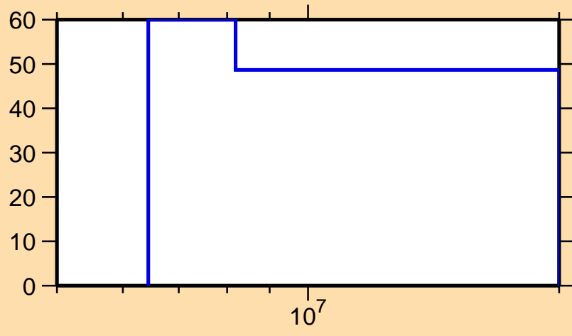
\Delta\sigma/\sigma vs. E for ^{151}\text{Pr}(n,\text{el.})
