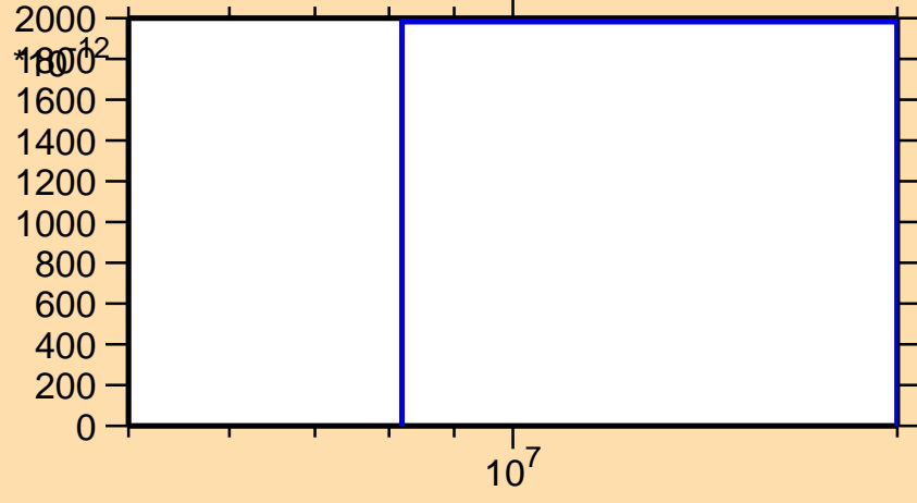
\sigma vs. E for ^{151}\text{Pr}(n,\text{nd})
