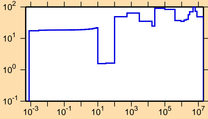
\Delta\sigma/\sigma vs. E for ^{151}\text{Pr}(n,\text{el.})
