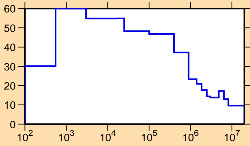
\Delta\sigma/\sigma vs. E for ^{151}\text{Pr}(n,\text{nonel.})
