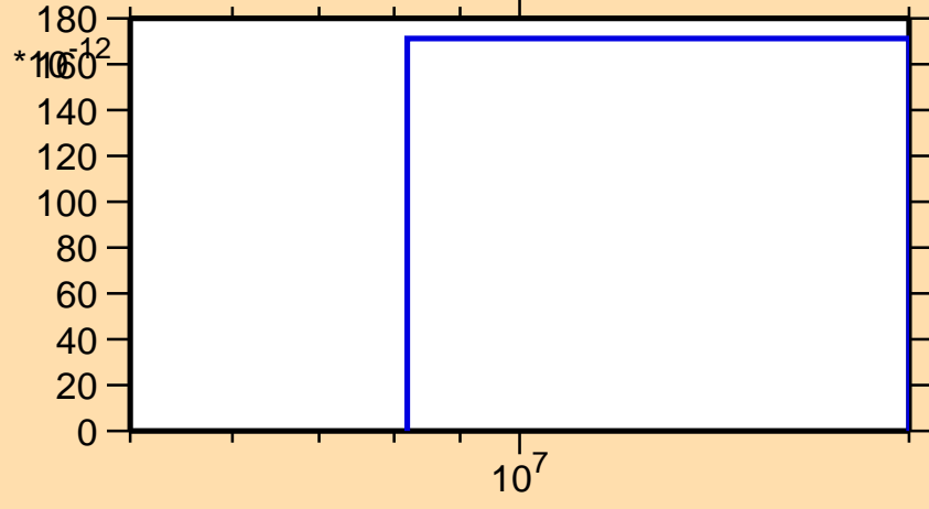
\sigma vs. E for ^{151}\text{Pr}(n,2n\alpha)
