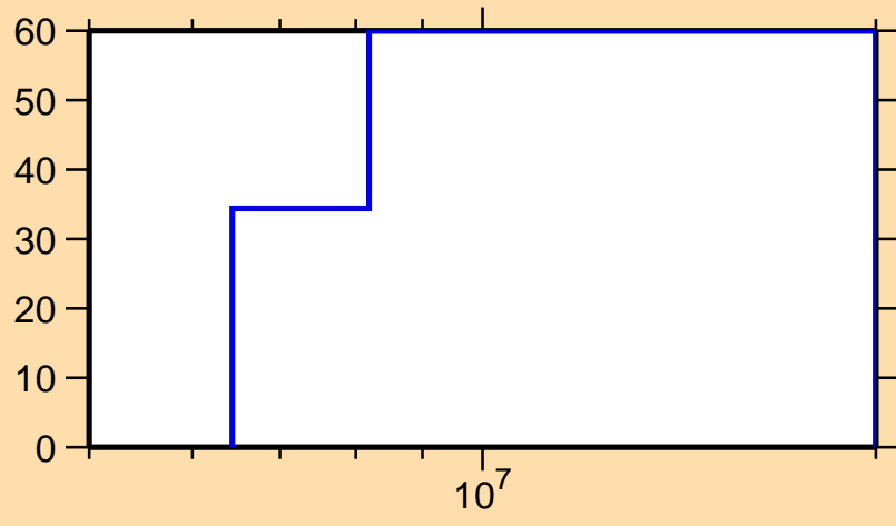
\Delta\sigma/\sigma vs. E for ^{151}\text{Pr}(n,2n)
