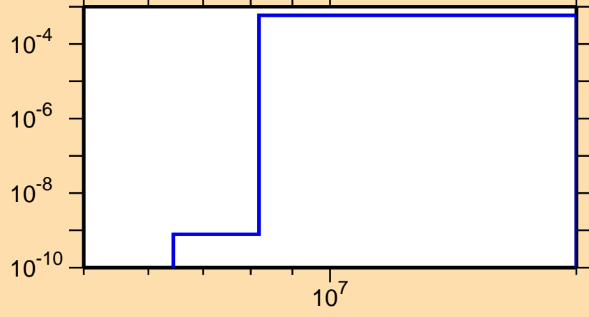
\sigma vs. E for ^{151}\text{Pr}(n,p)
