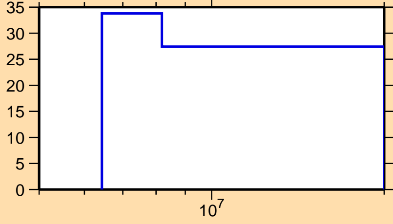
\Delta\sigma/\sigma vs. E for ^{151}\text{Pr}(n,\text{tot.})
