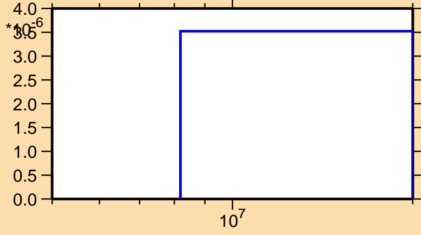
\sigma vs. E for ^{151}\text{Pr}(n,n\alpha)
