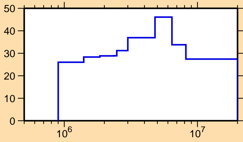
\Delta\sigma/\sigma vs. E for ^{151}\text{Pr}(n,\text{tot.})
