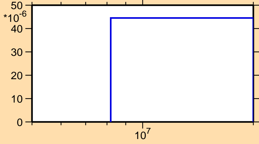
\sigma vs. E for ^{151}\text{Pr}(n,d)
