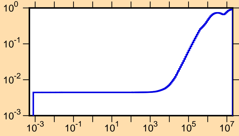
\mu vs. E for ^{152}\text{Pr}(\text{mt251})
