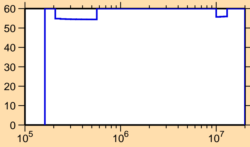
\Delta\sigma/\sigma vs. E for ^{152}\text{Pr}(n,n_1)
