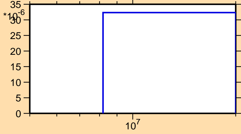
\sigma vs. E for ^{152}\text{Pr}(n,d)
