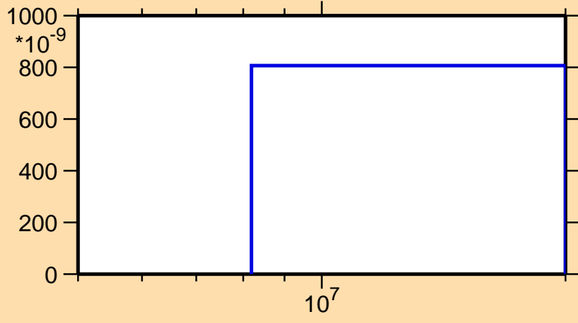
\sigma vs. E for ^{152}\text{Pr}(n,n\alpha)
