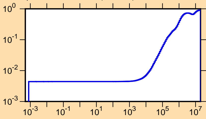
\mu vs. E for ^{153}\text{Pr}(\text{mt251})
