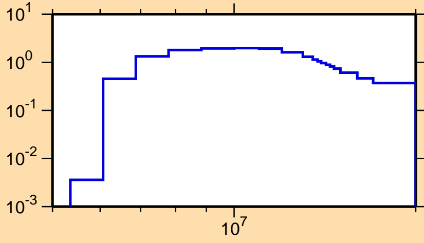
\sigma vs. E for ^{153}\text{Pr}(n,2n)
