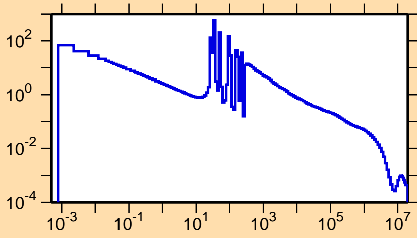
\sigma vs. E for ^{153}\text{Pr}(n,\gamma)
