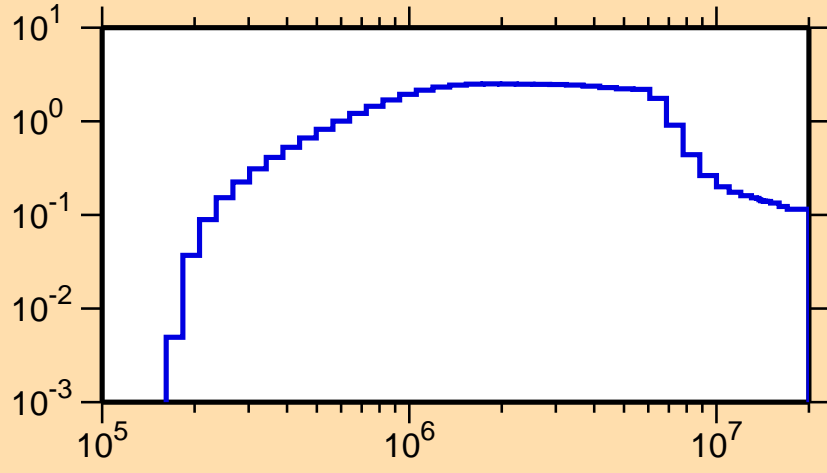
\sigma vs. E for ^{153}\text{Pr}(n,n\text{cont.})
