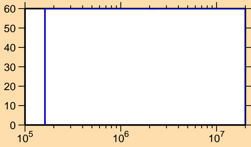
\Delta\sigma/\sigma vs. E for ^{153}\text{Pr}(n,n_1)
