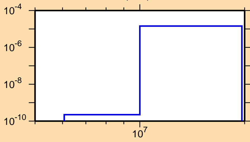
\sigma vs. E for ^{153}\text{Pr}(n,\alpha)
