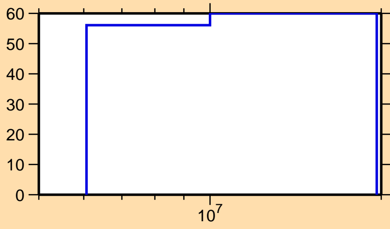
\Delta\sigma/\sigma vs. E for ^{153}\text{Pr}(n,p)
