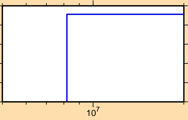
\sigma vs. E for ^{153}\text{Pr}(n,d)
