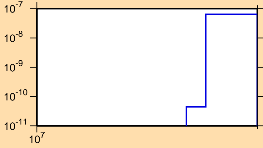
\sigma vs. E for ^{154}\text{Pr}(n,2np)
