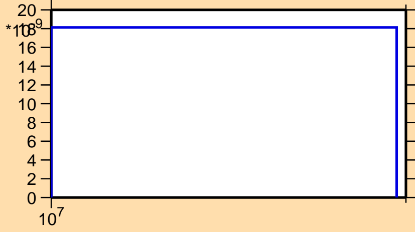
\sigma vs. E for ^{154}\text{Pr}(n,\text{nd})
