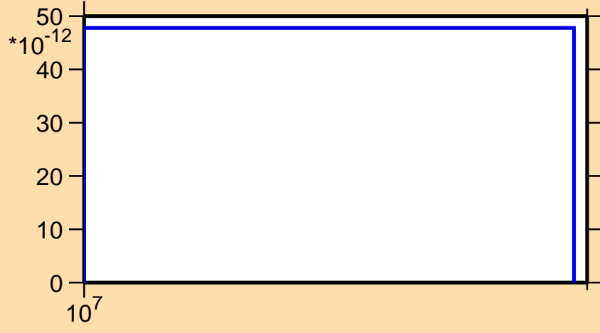
\sigma vs. E for ^{154}\text{Pr}(n,2n\alpha)
