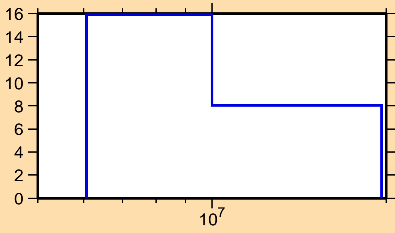
\Delta\sigma/\sigma vs. E for ^{154}\text{Pr}(n,el.)
