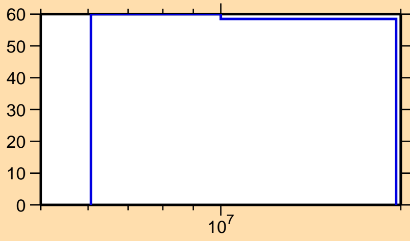
\Delta\sigma/\sigma vs. E for ^{154}\text{Pr}(n,n_1)
