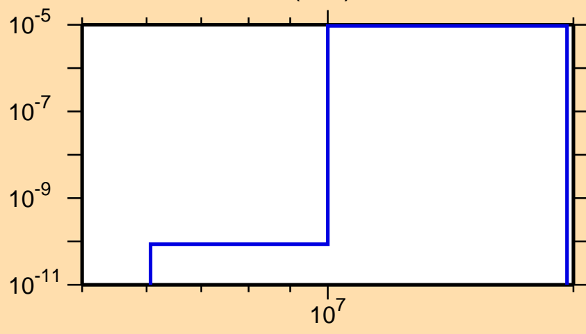
\sigma vs. E for ^{154}\text{Pr}(n,\alpha)
