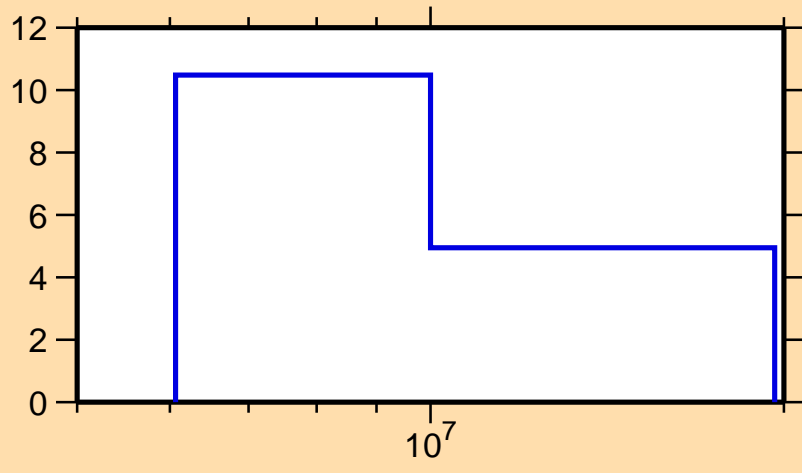
\Delta\sigma/\sigma vs. E for ^{154}\text{Pr}(n,\text{tot.})
