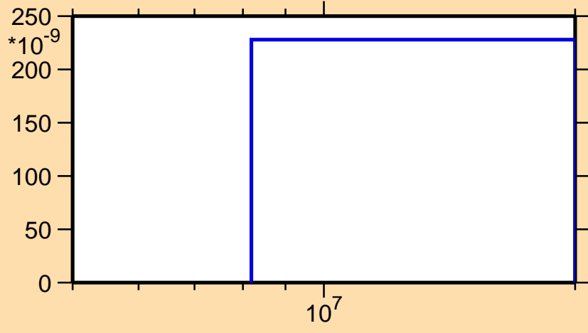
\sigma vs. E for ^{154}\text{Pr}(n,n\alpha)
