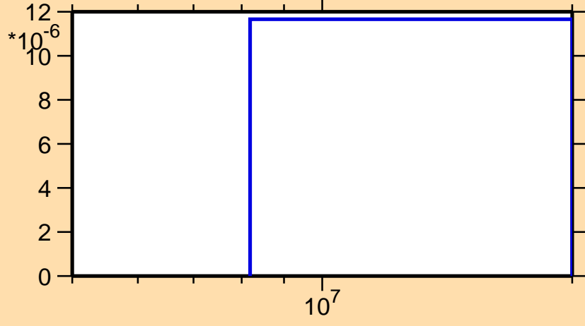
\sigma vs. E for ^{154}\text{Pr}(n,d)
