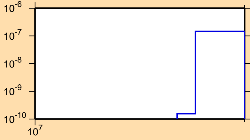
\sigma vs. E for ^{155}\text{Pr}(n,\text{nd})
