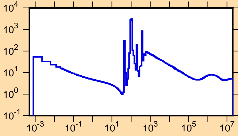
\sigma vs. E for ^{155}\text{Pr}(n,\text{tot.})
