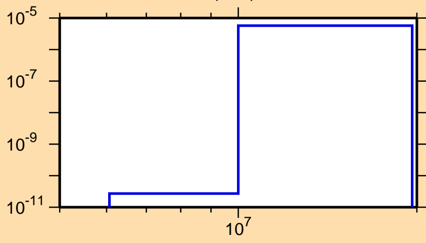
\sigma vs. E for ^{155}\text{Pr}(n,\alpha)
