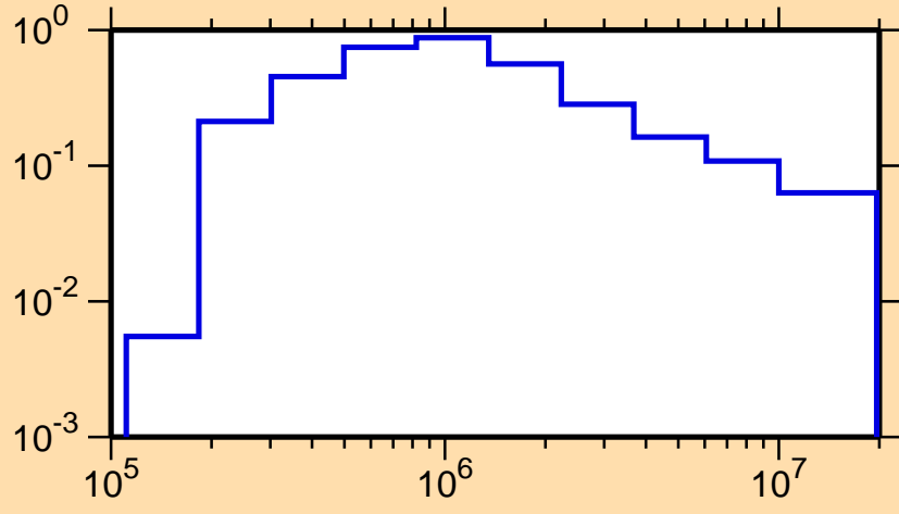
\sigma vs. E for ^{155}\text{Pr}(n,n_1)
