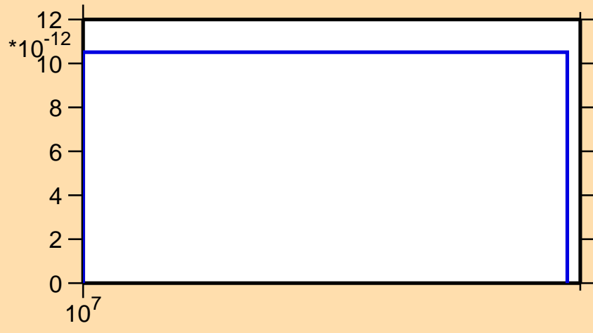
\sigma vs. E for ^{155}\text{Pr}(n,2np)
