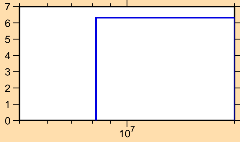
\Delta\sigma/\sigma vs. E for ^{155}\text{Pr}(n,\text{nonel.})
