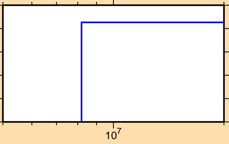
\sigma vs. E for ^{155}\text{Pr}(n,np)
