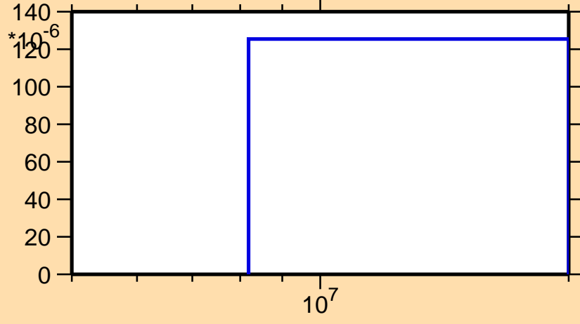
\sigma vs. E for ^{155}\text{Pr}(n,p)
