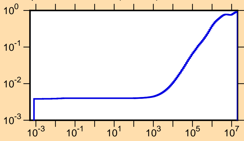
\mu vs. E for ^{176}\text{Pt}(\text{mt251})
