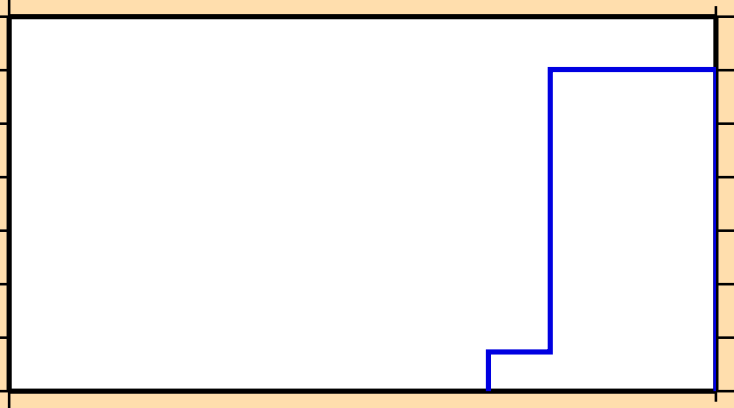
\sigma vs. E for ^{176}\text{Pt}(n,nt)
