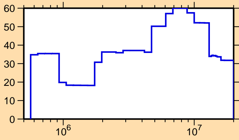
\Delta\sigma/\sigma vs. E for ^{176}\text{Pt}(n, el.)
