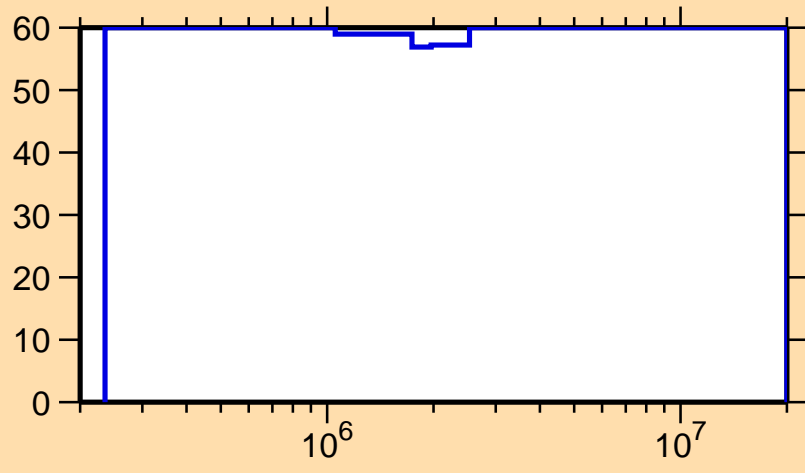
\Delta\sigma/\sigma vs. E for ^{176}\text{Pt}(n,n_1)
