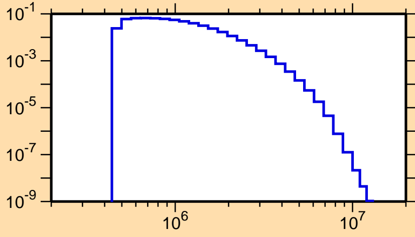
\sigma vs. E for ^{176}\text{Pt}(n,n_2)
